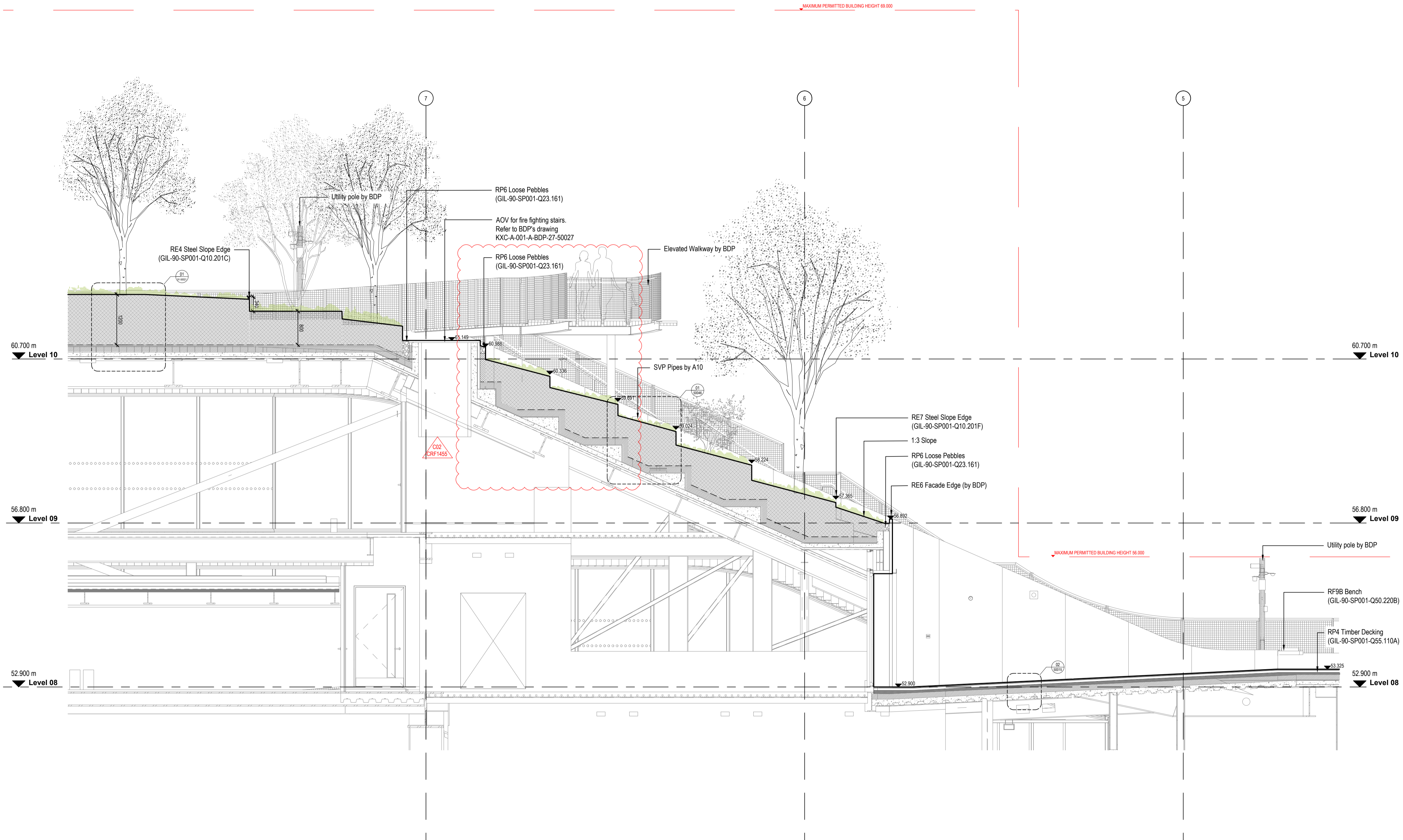
01 Section - Garden to Headland Slope Scale 1:50 @ A1
