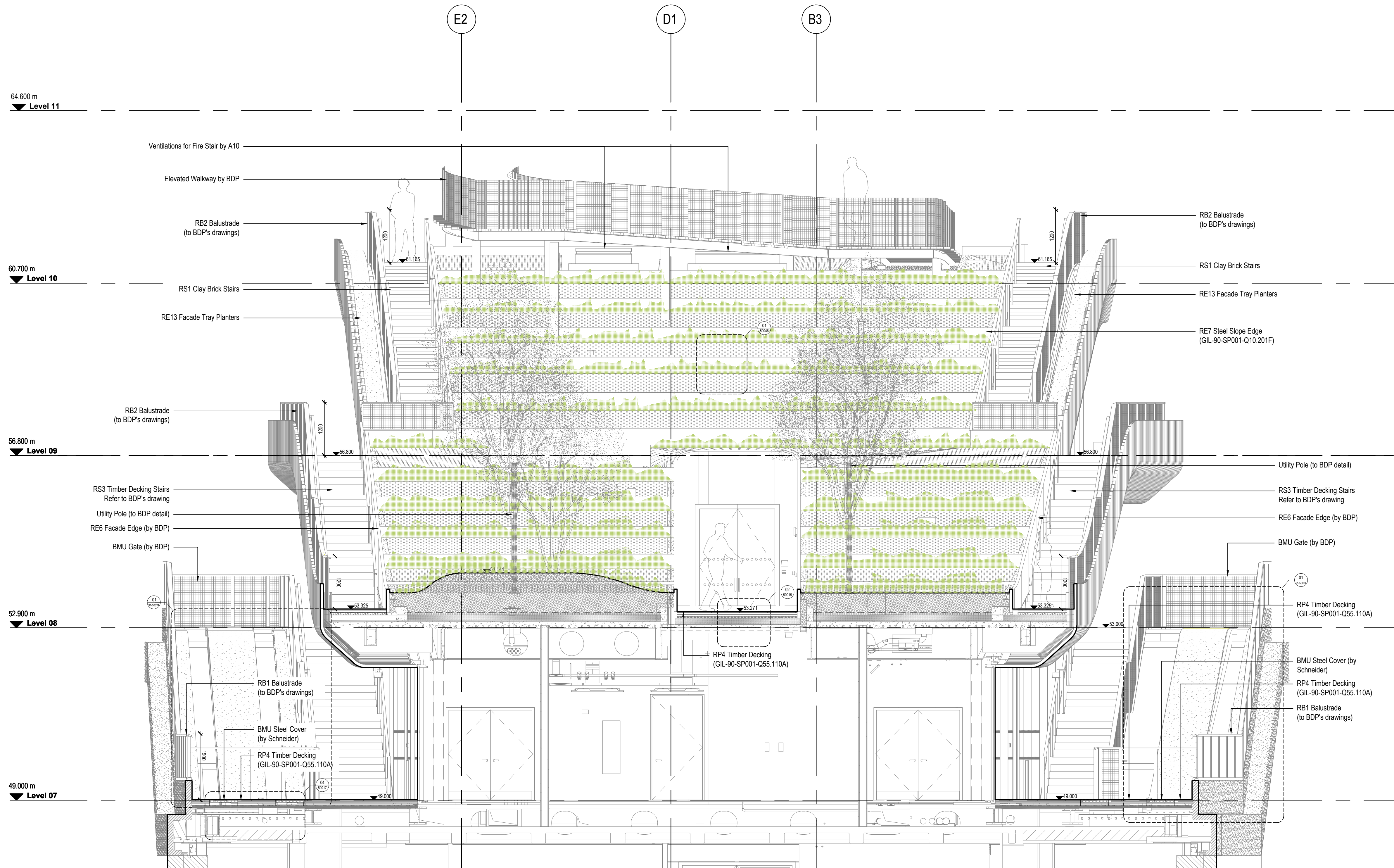
01 20051 Section - Headland Scale 1:50 @ A1
