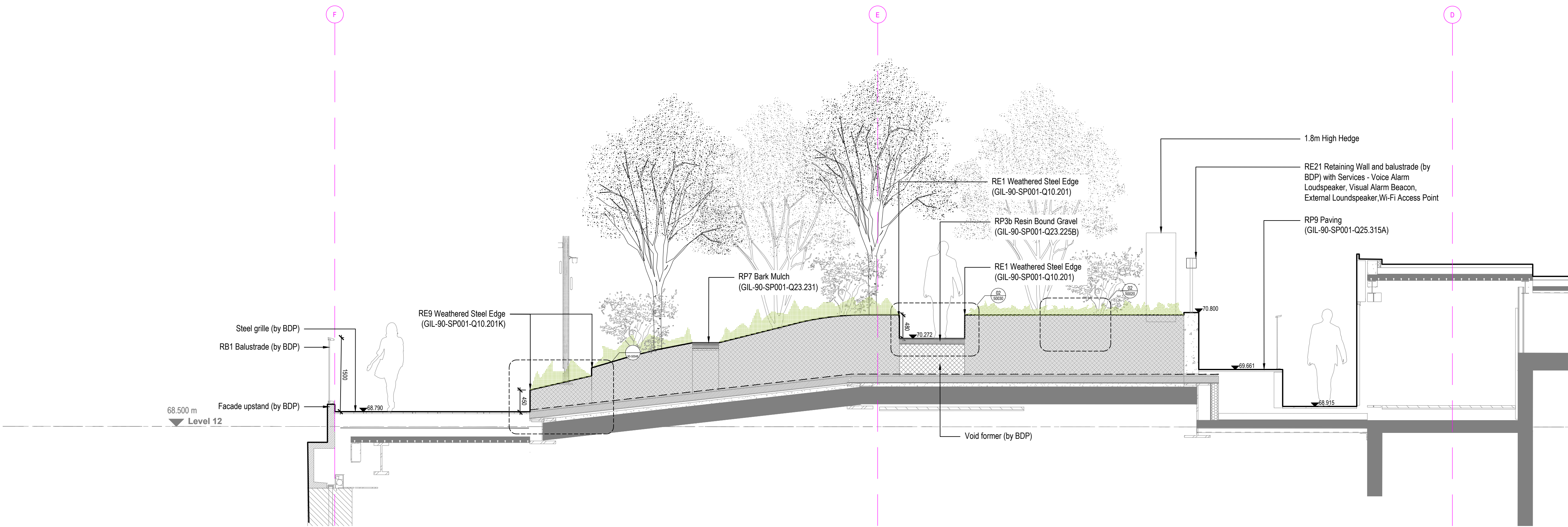
01 20043 Section - Plateau - Gridline 30 Scale 1:50 @ A1
