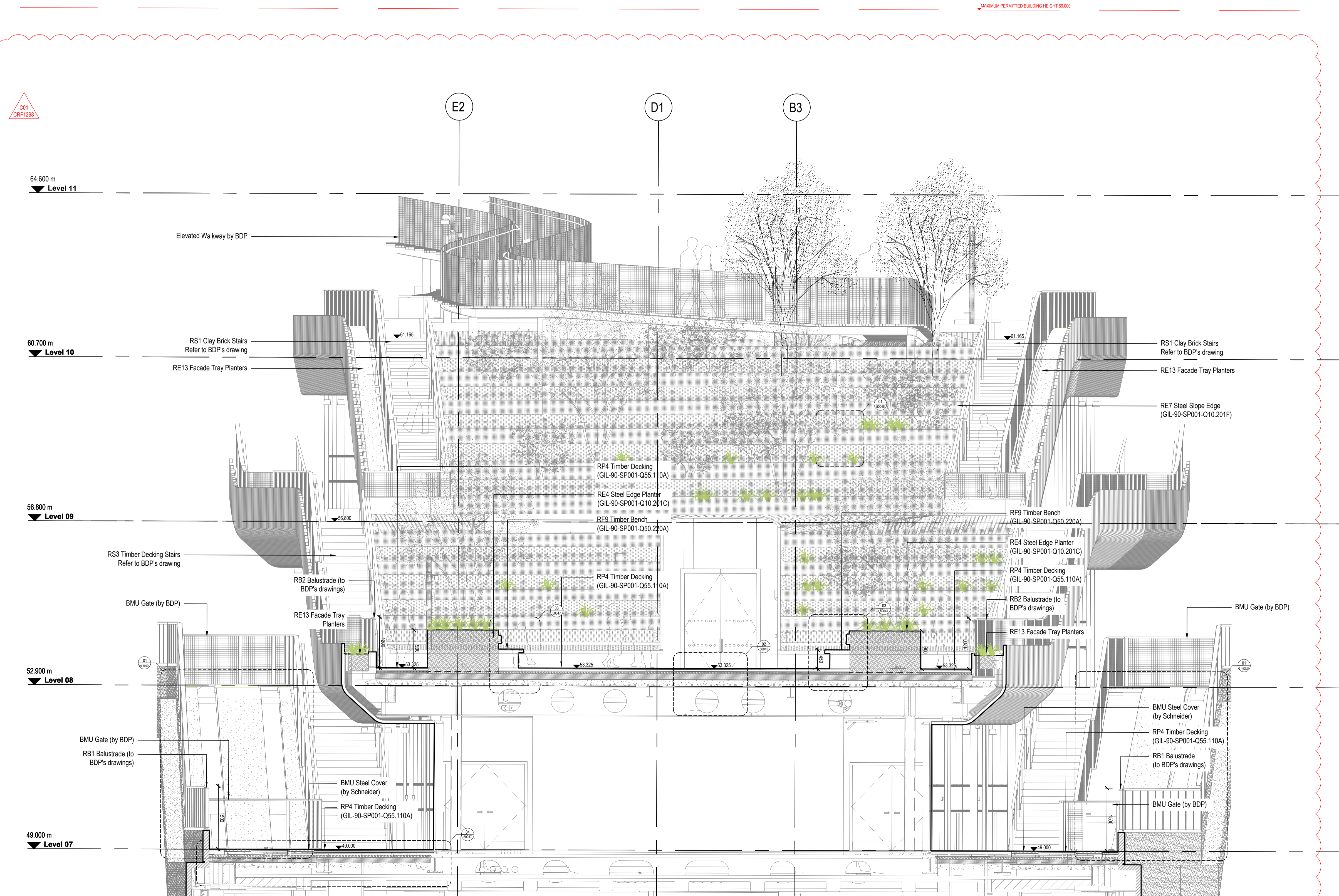
02 20040 Section - Headland - Gridline 4 Scale 1:50 @ A1
