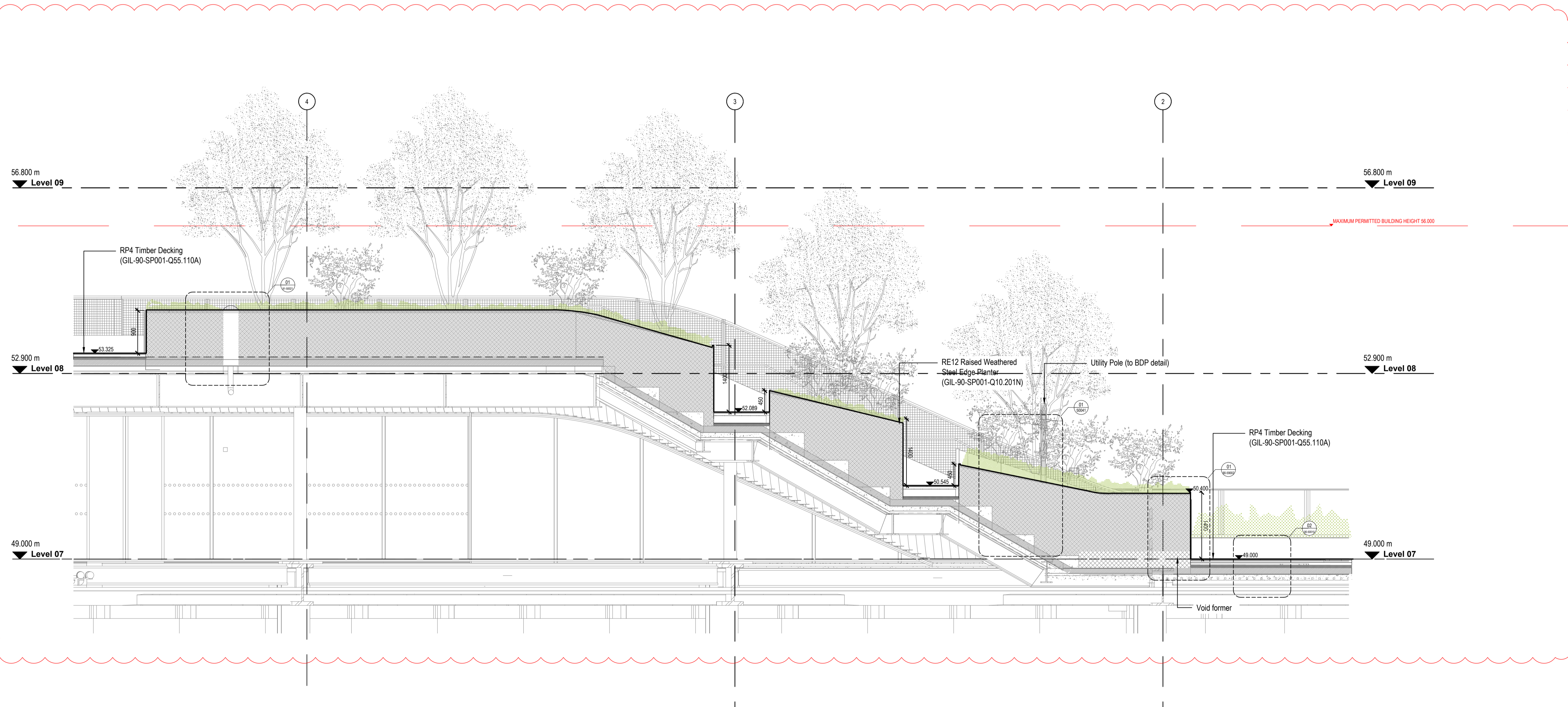
01 20009 Section - Headland Slope Scale 1:50 @ A1
