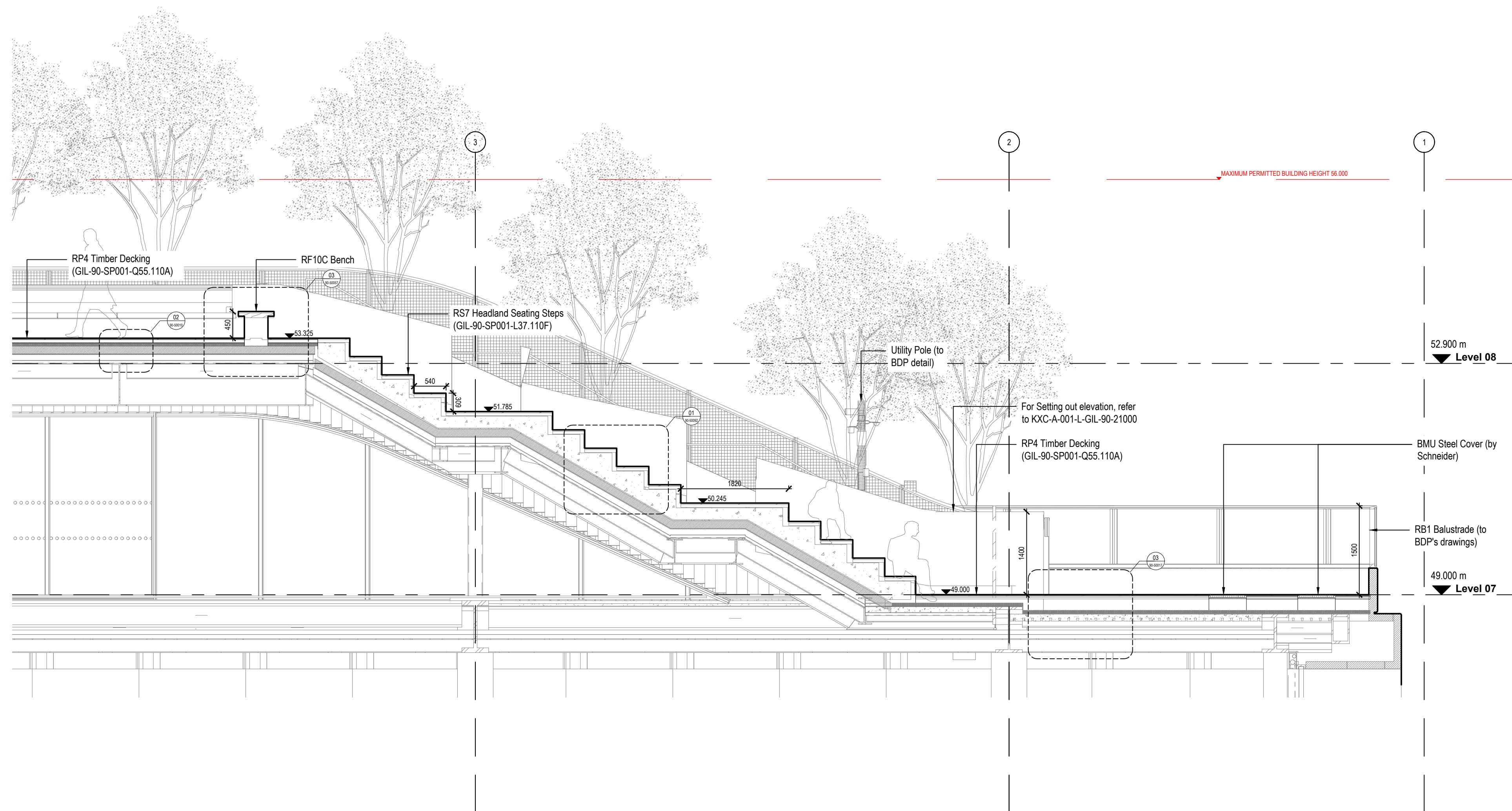
01 20008 Section - Headland Slope Scale 1:50 @ A1
