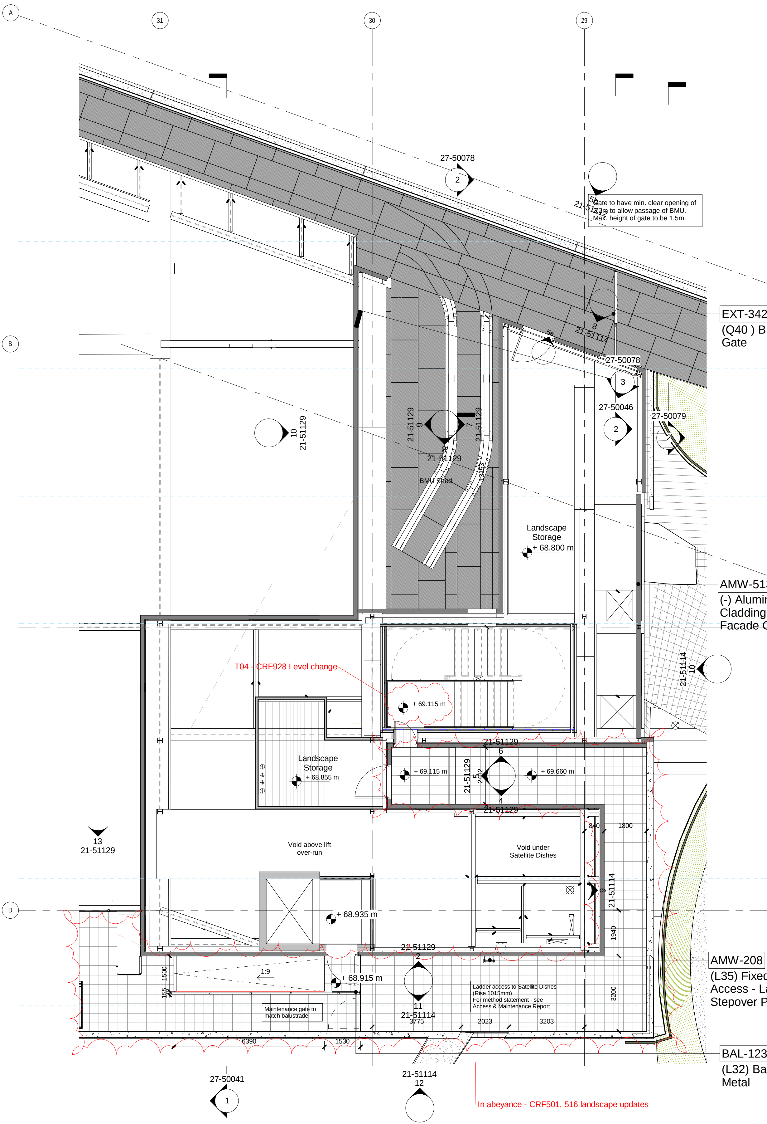
1 North Shed 1:100
