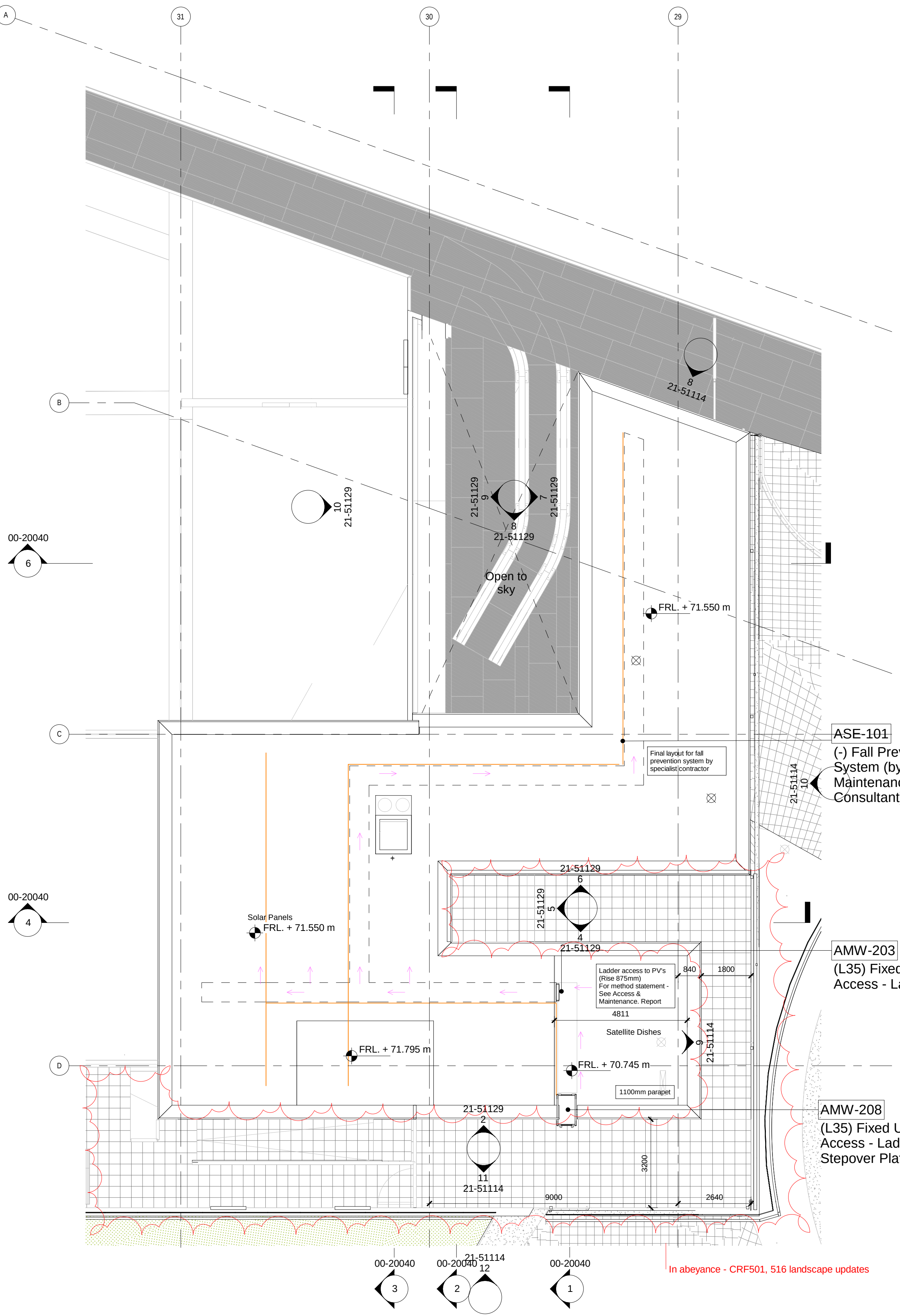
2 North Shed Roof 1:100
