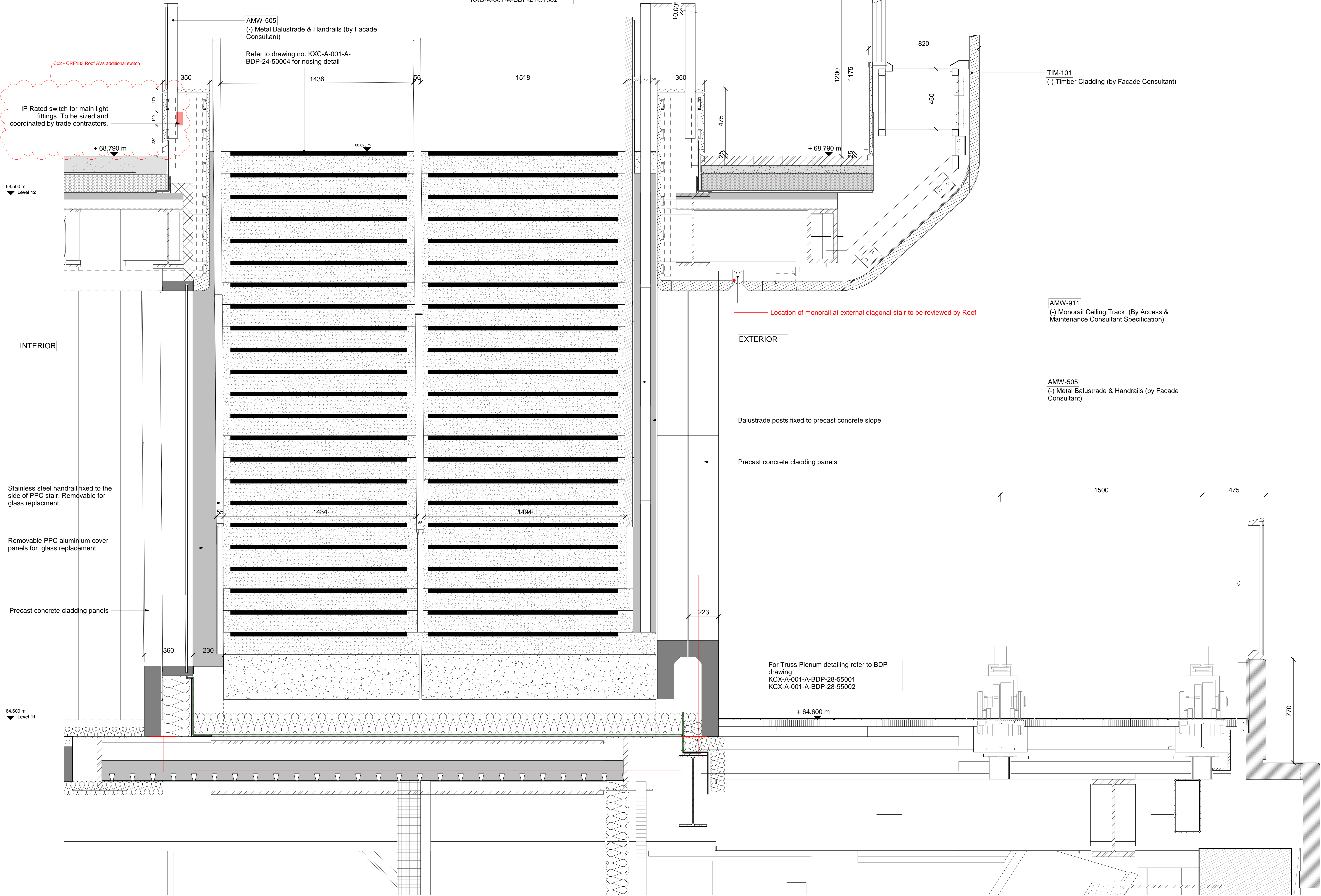
4 Cross Section - Roof Diagonal Stair 1:10
