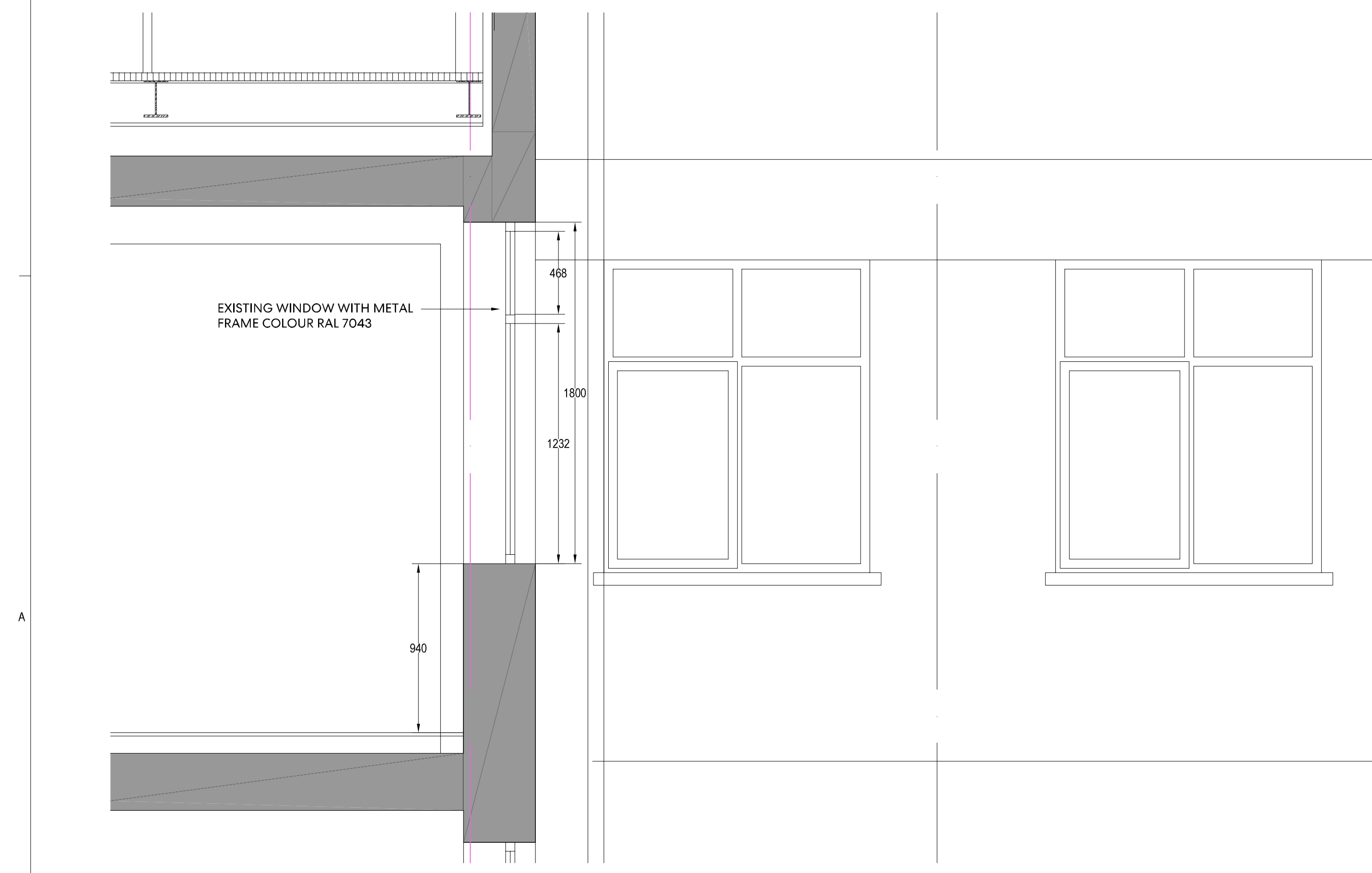
2 ENLARGED EXISTING SECTION - LEVEL 03 1:20
