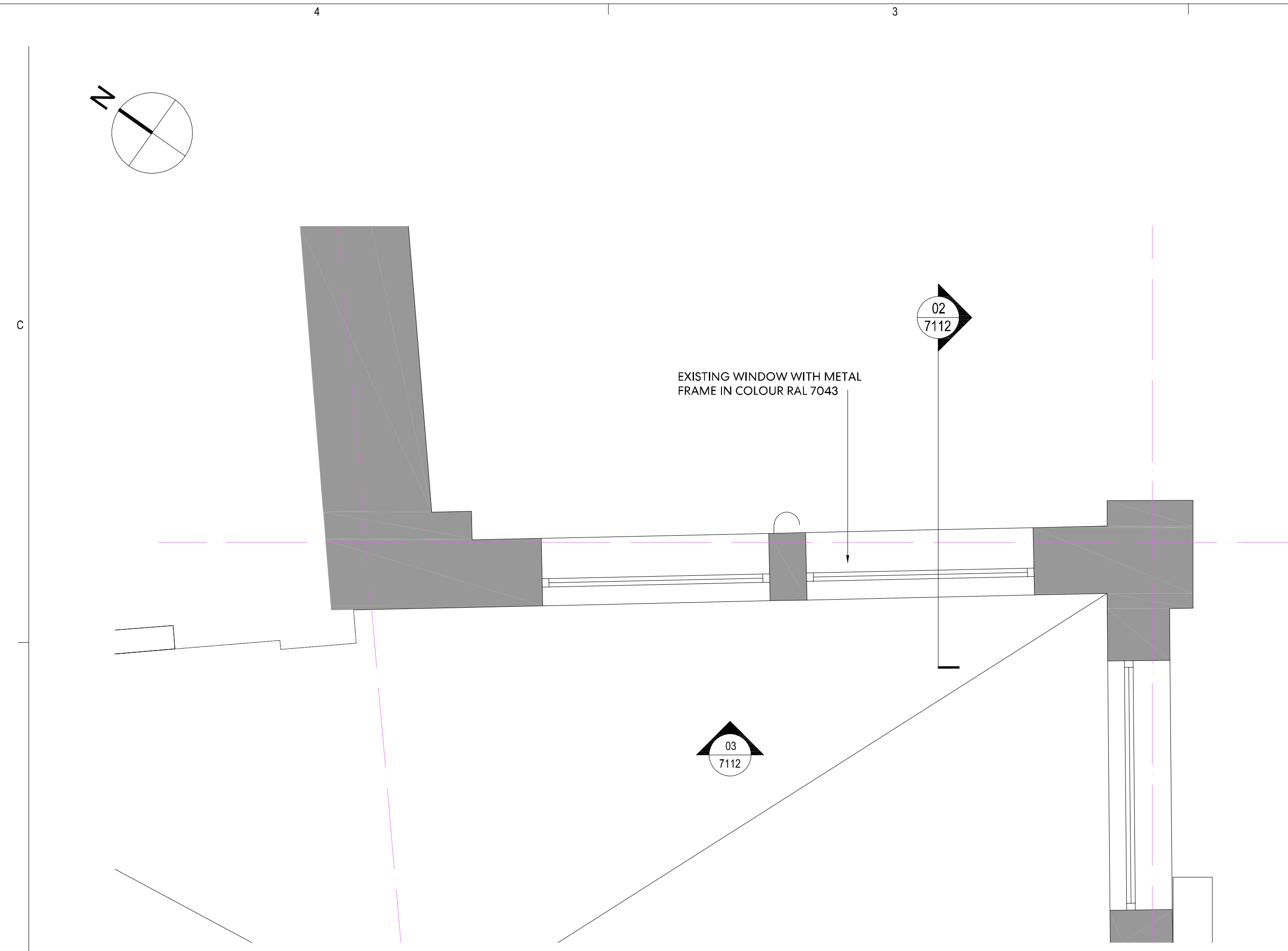
1 ENLARGED EXISTING GENERAL ARRANGEMENT PLAN - LEVEL 03 1:20
