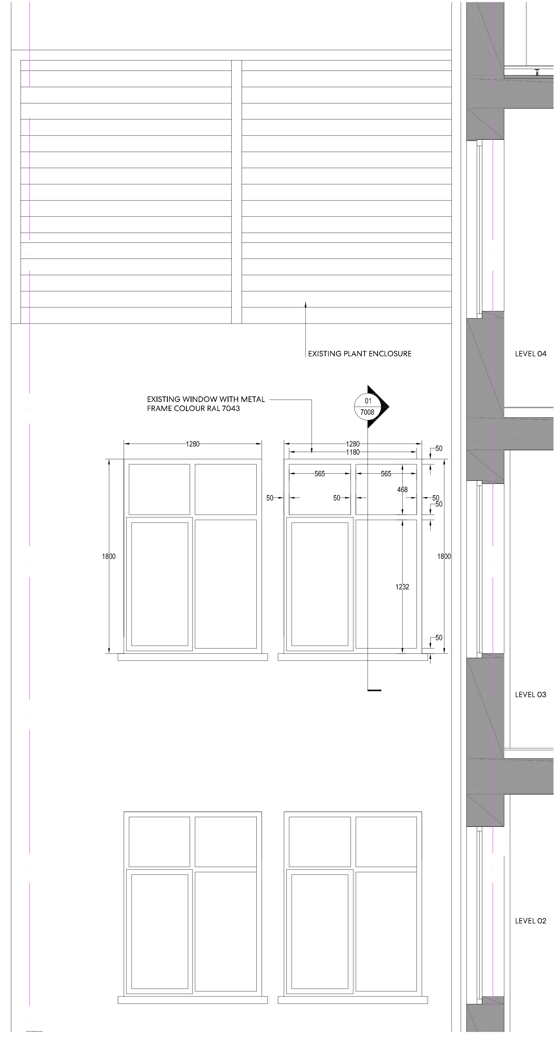
3 ENLARGED EXISTING INTERNAL ELEVATION - LEVEL 03 1:20
