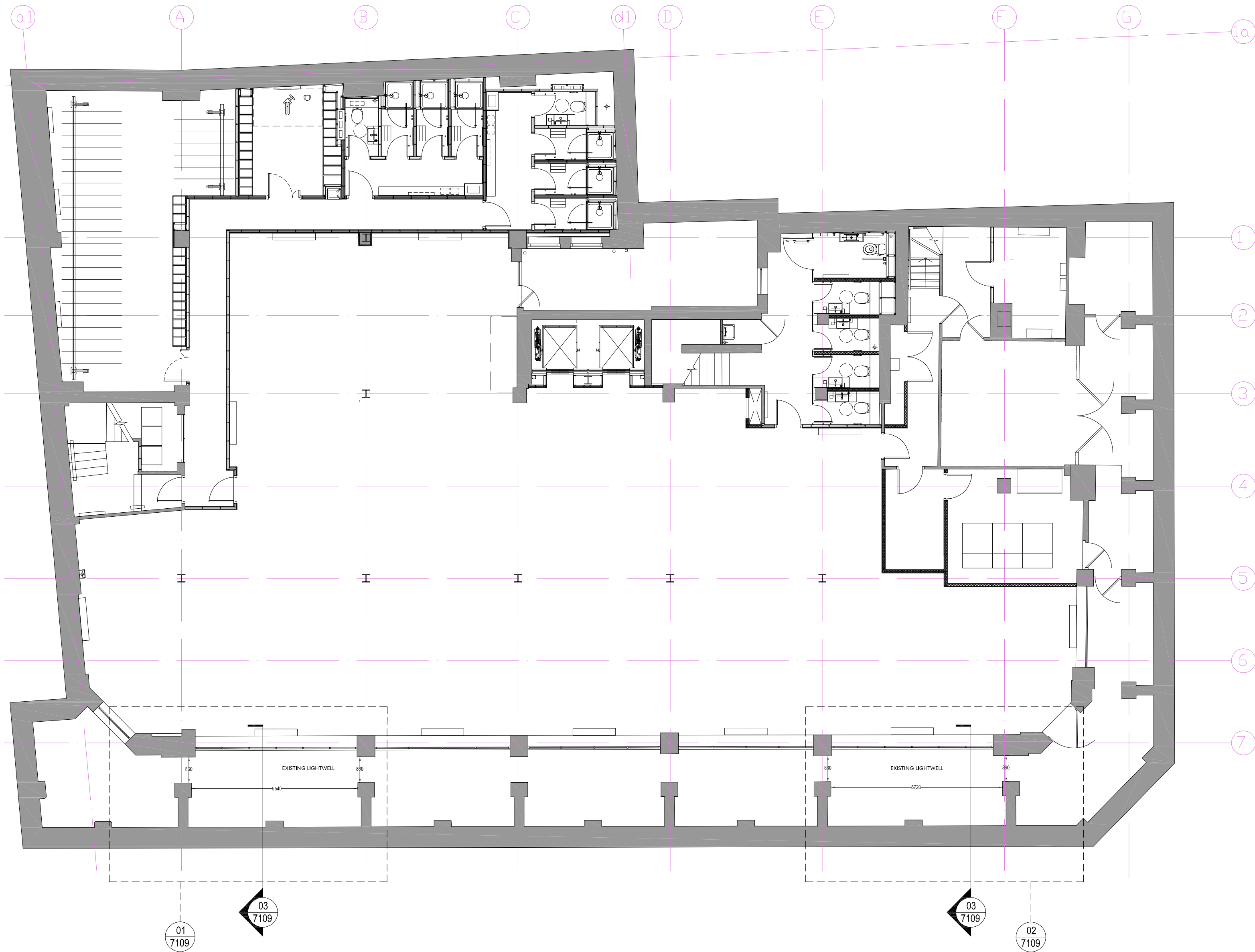
1 EXISTING GENERAL ARRANGEMENT PLAN - LEVEL B1 1 : 100
