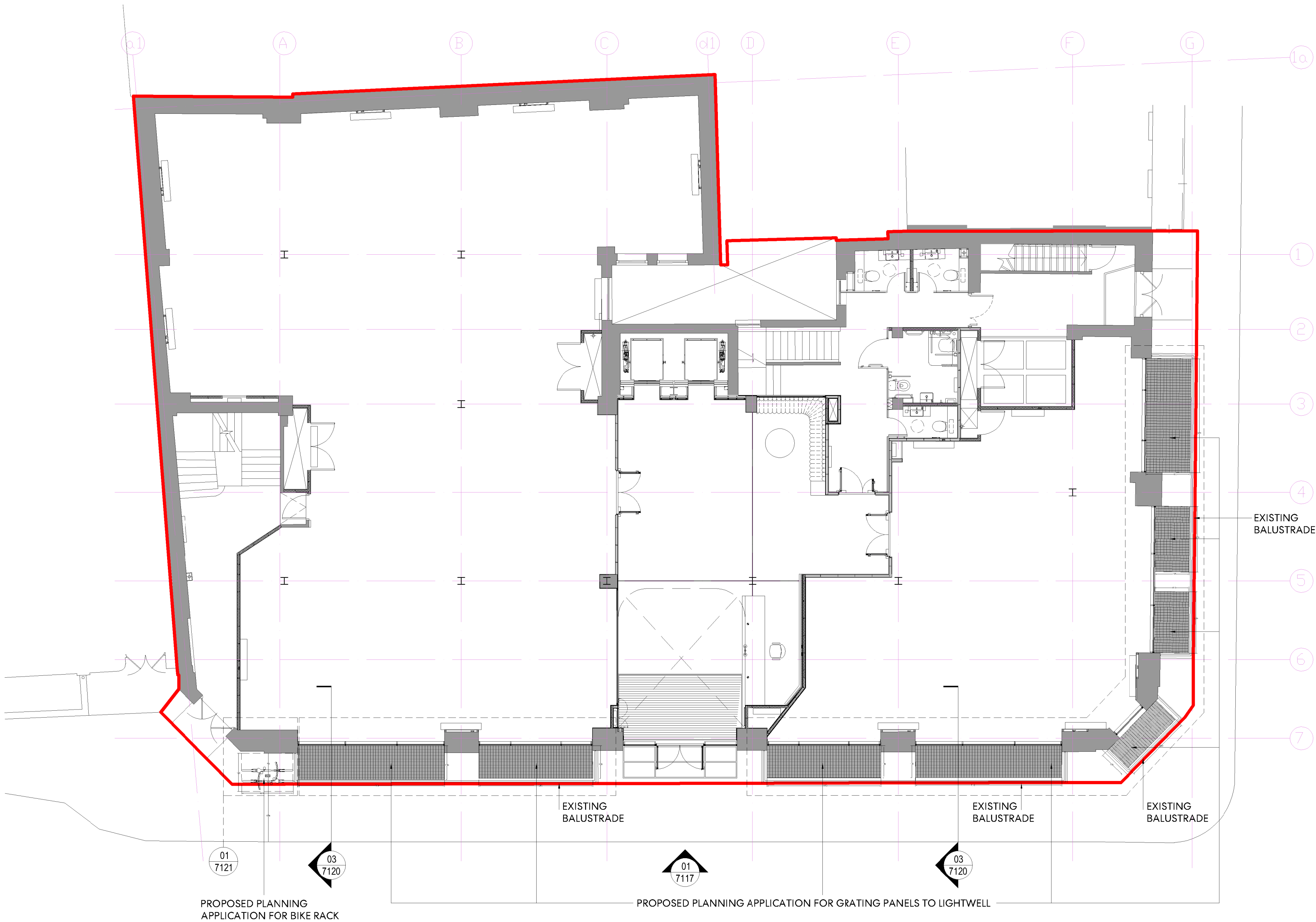
1 PROPOSED GENERAL ARRANGEMENT PLAN - LEVEL 00 1 : 100
