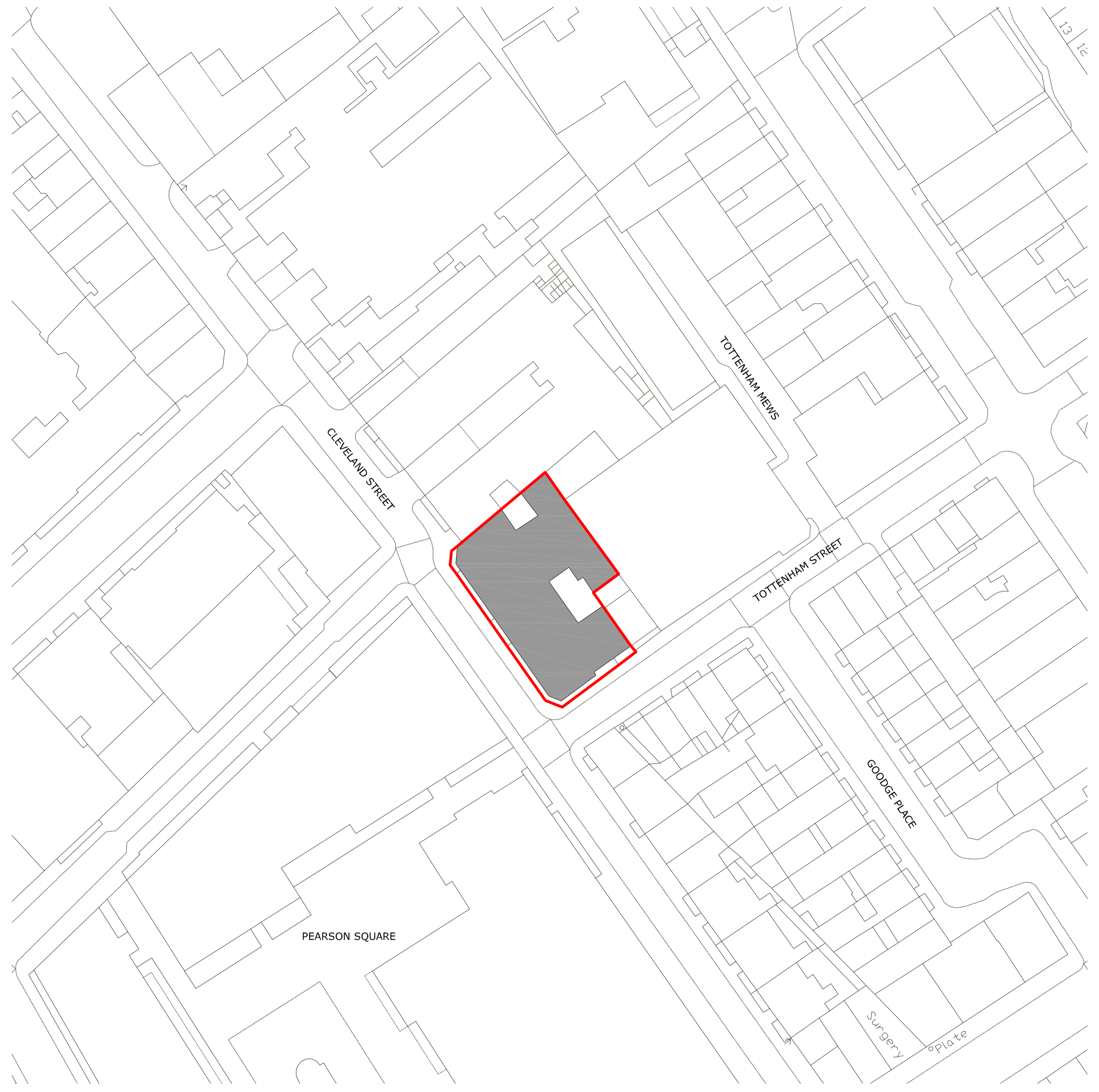
1 PLANNING - LEVEL 00 SITE PLAN 1:500
