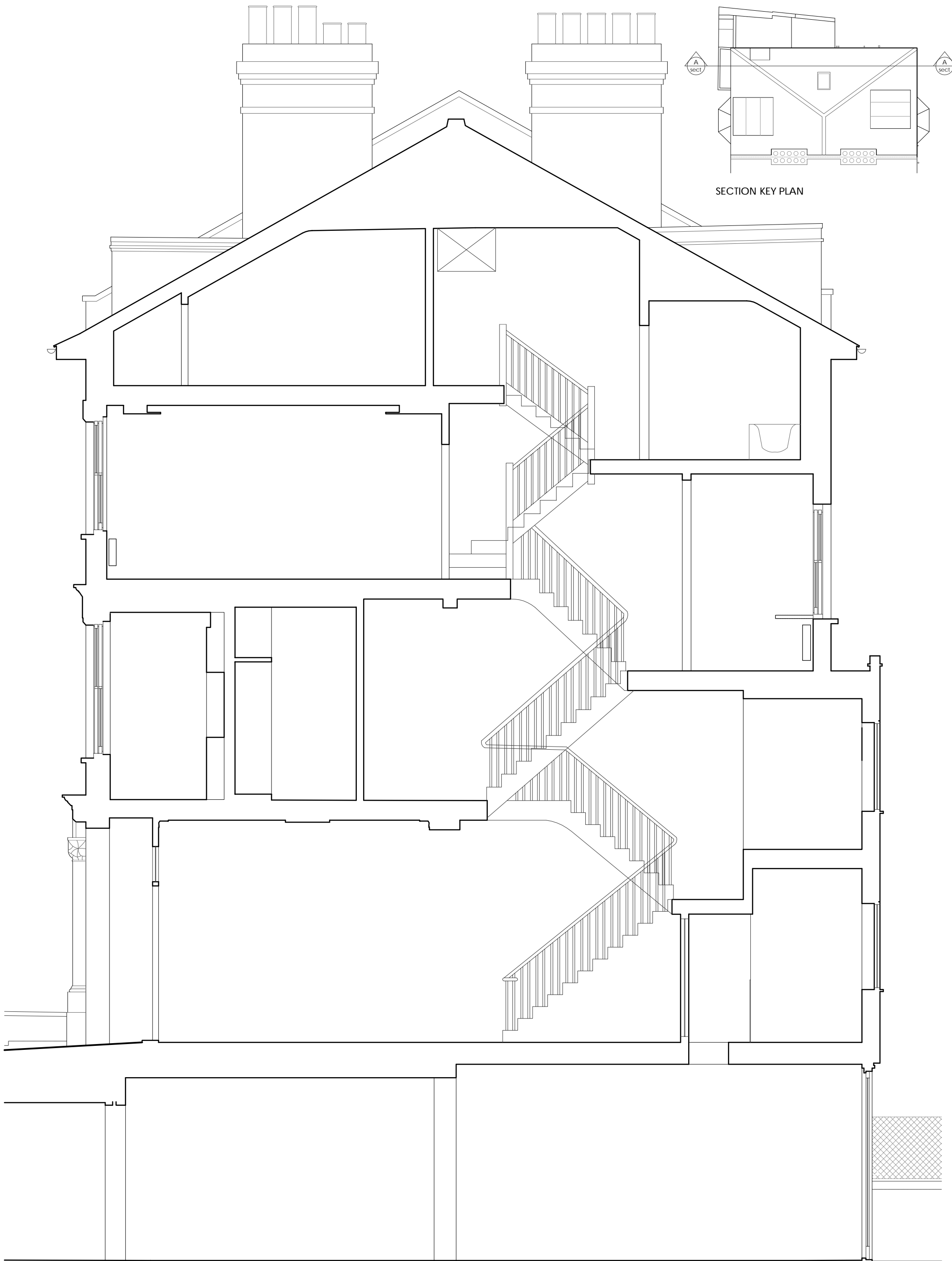
SECTION A-A - FRONT TO REAR
