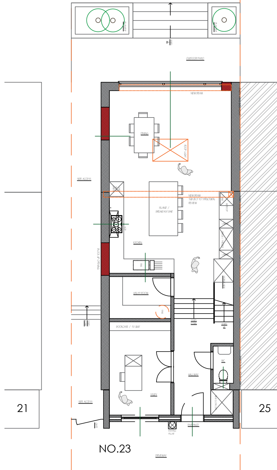
PLAN GROUND / BASEMENT FL. 1:100
