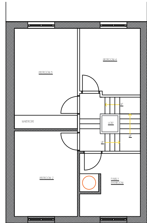
PLAN SECOND FLOOR 1:100
