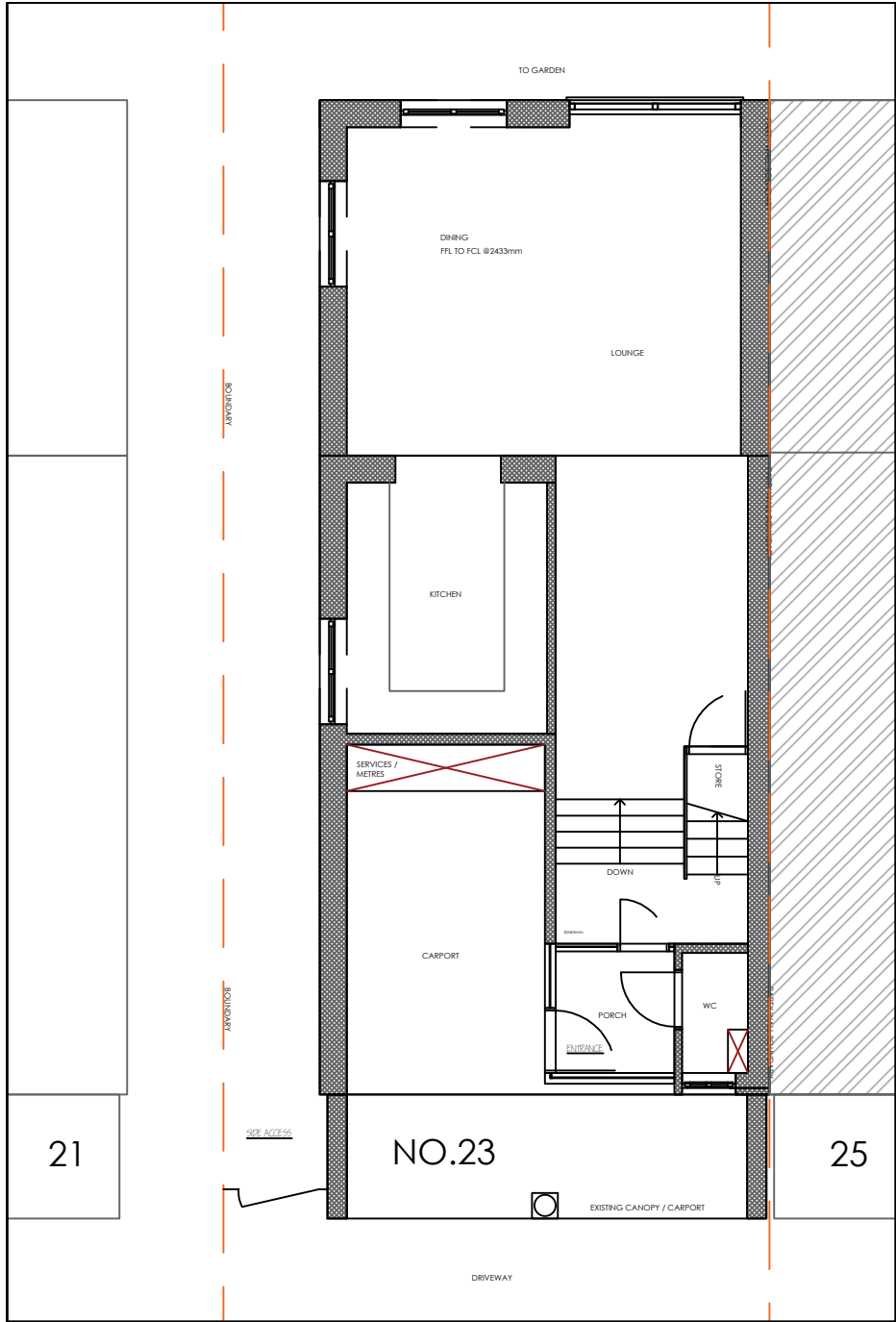
PLAN GROUND / BASEMENT FL. 1:100
