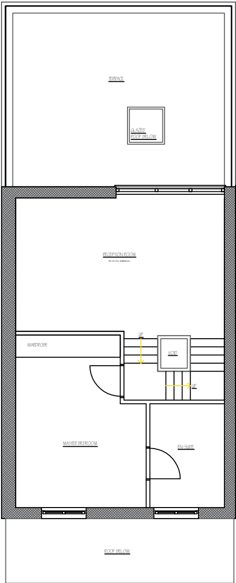
PLAN FIRST FLOOR 1:100
