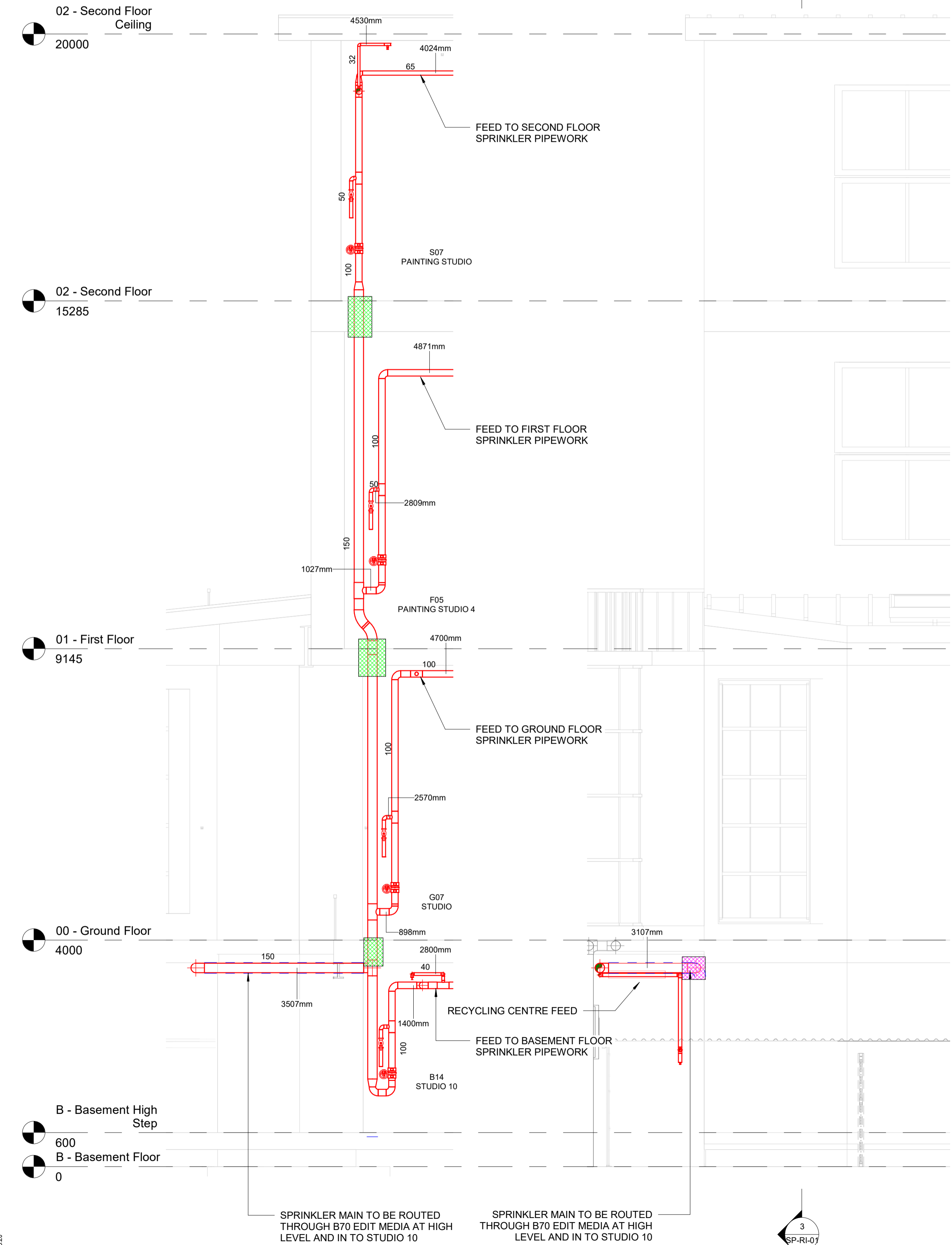
3 Riser Pipework Internal Section 1 1 : 50
