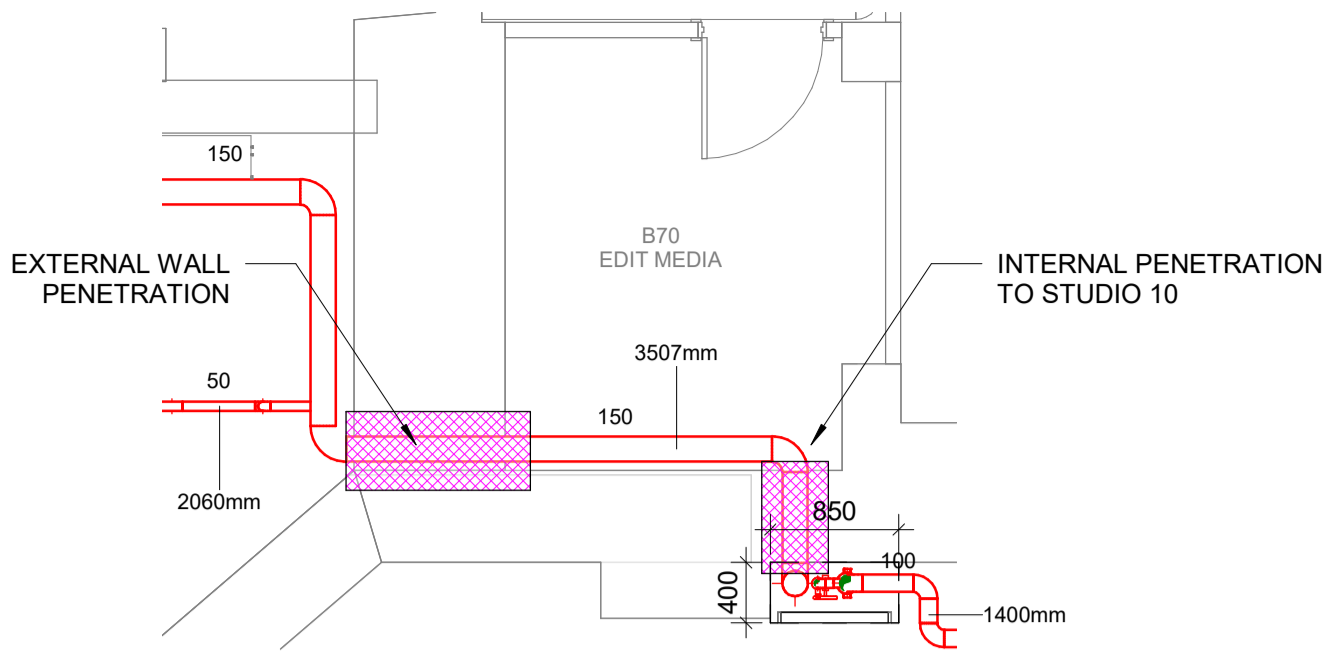
1 Riser Internal Basement & Ground Plan 1 : 50
