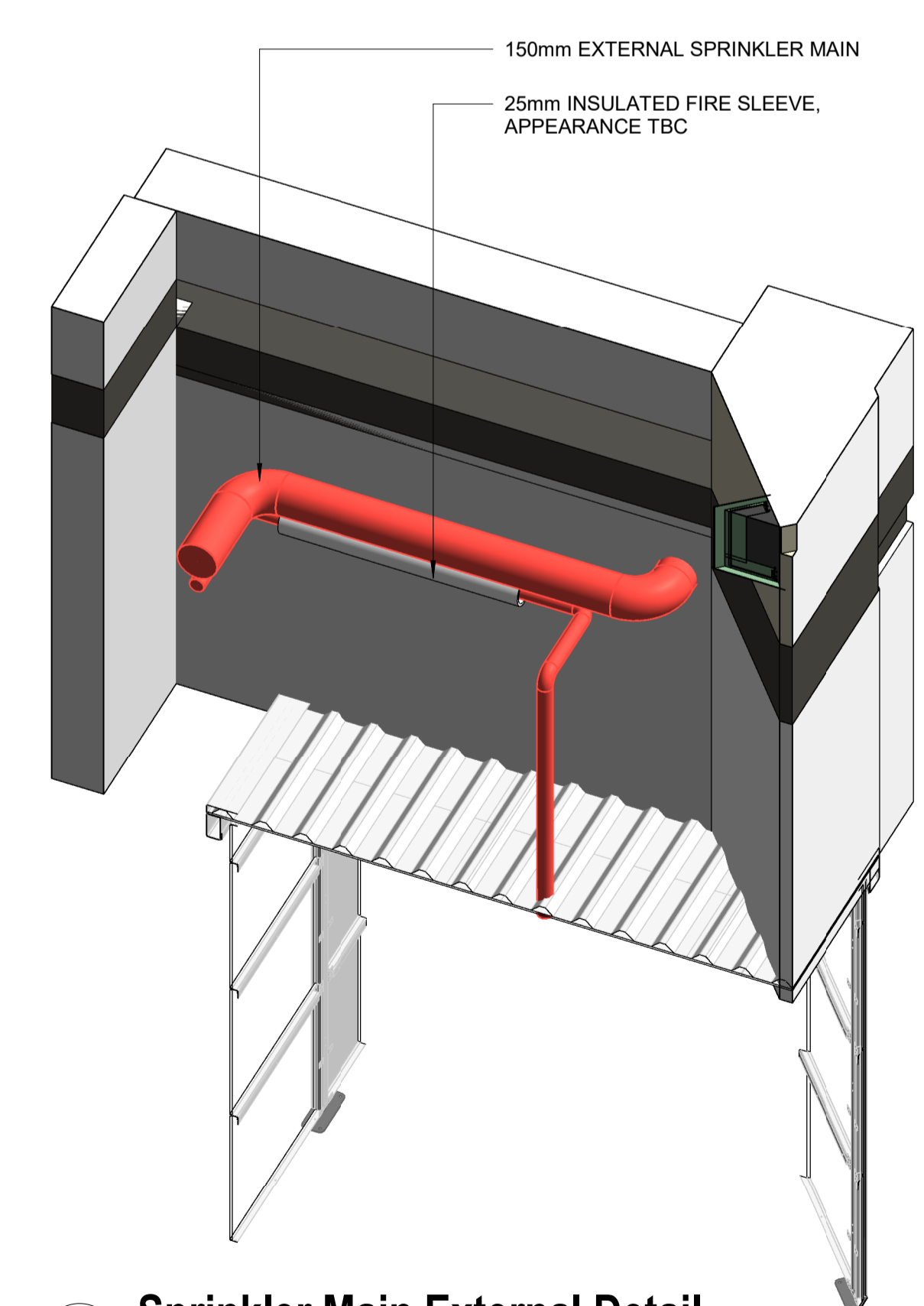
6 Sprinkler Main External Detail
