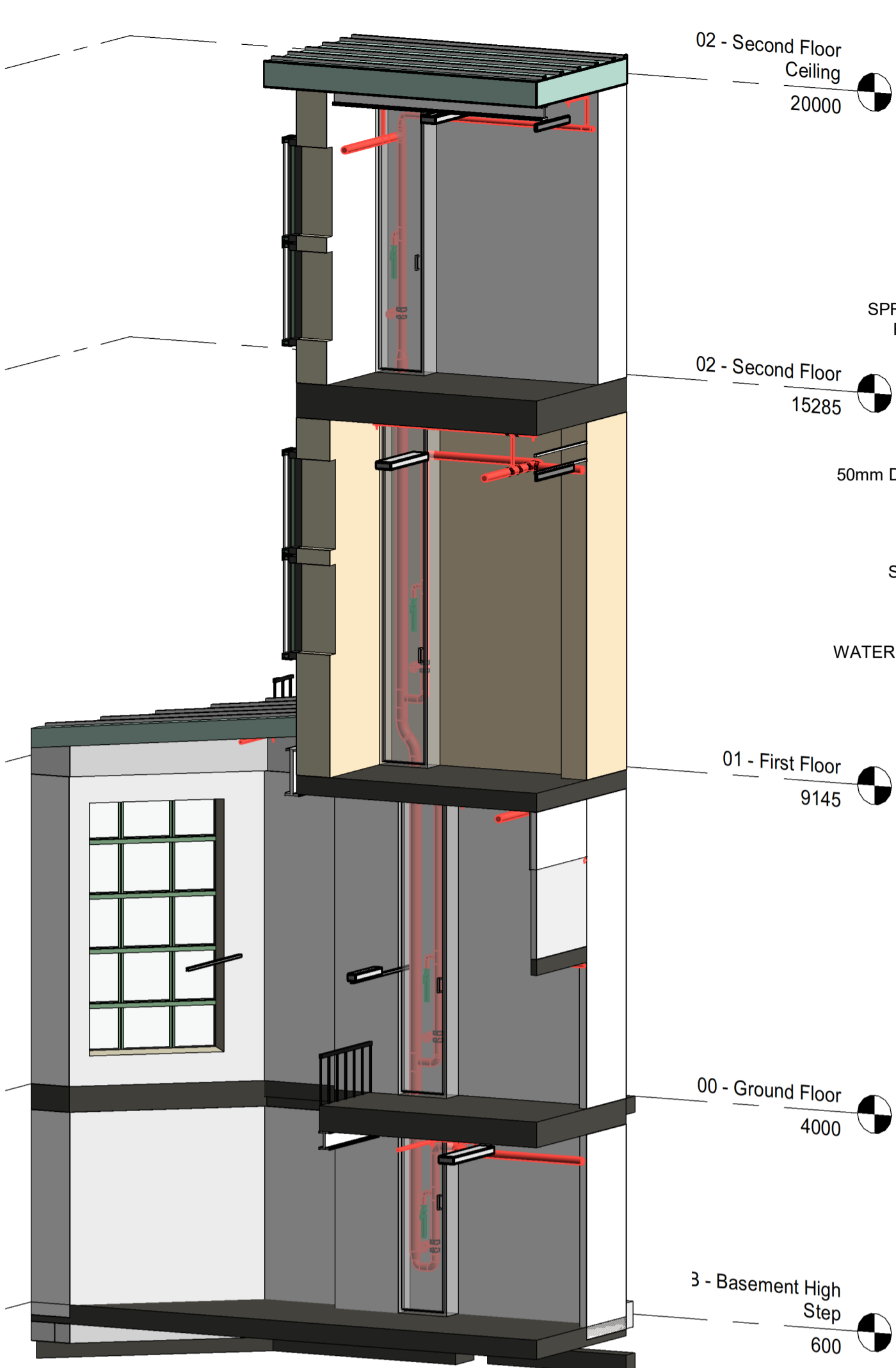
5 Riser Internal 3D
