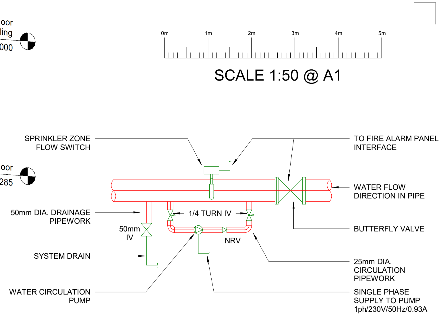
8 12 - Zone Control Arrangement Detail 1 : 10
