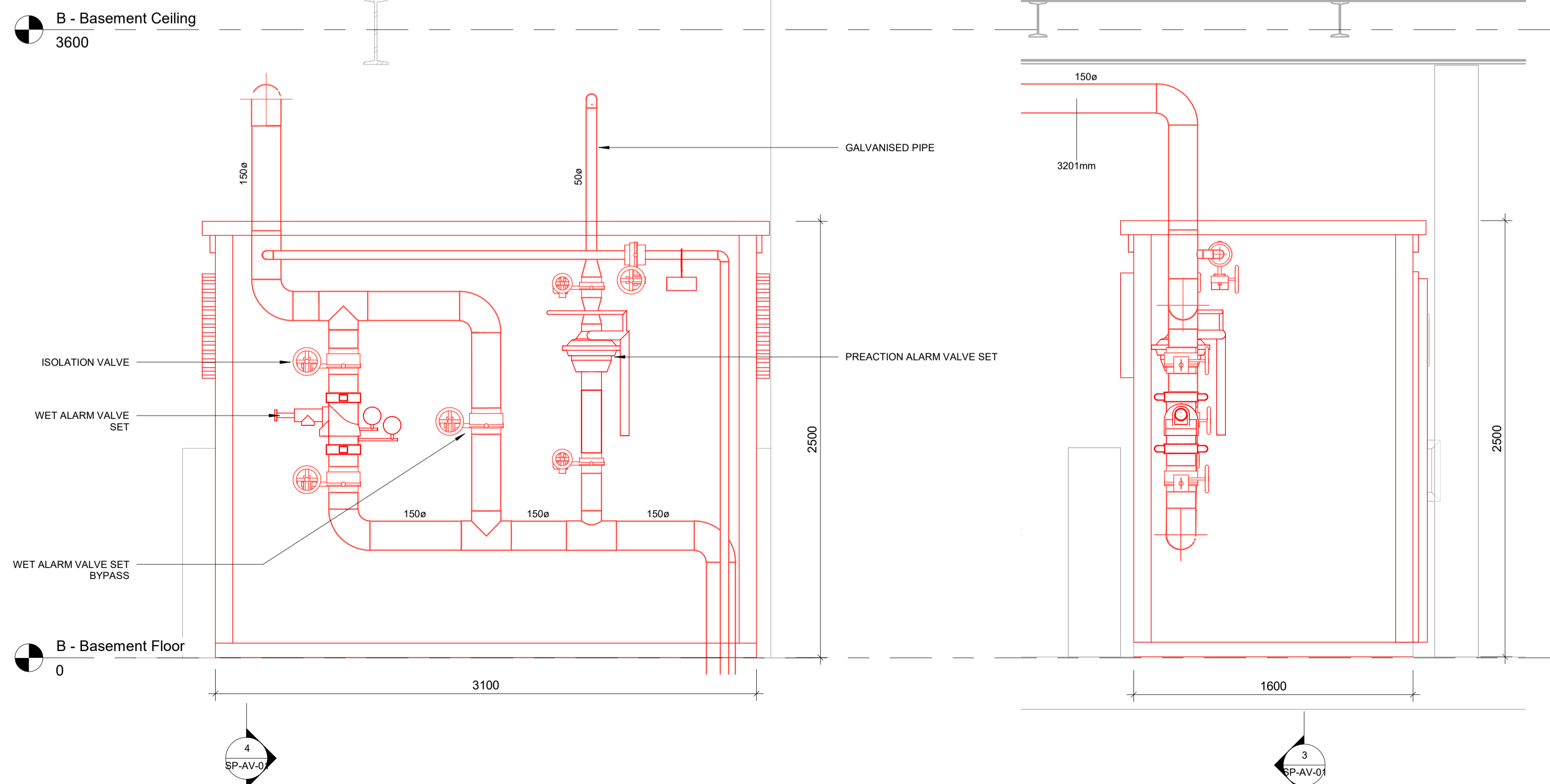
3 Alarm Valve Room Section 1 1:20
