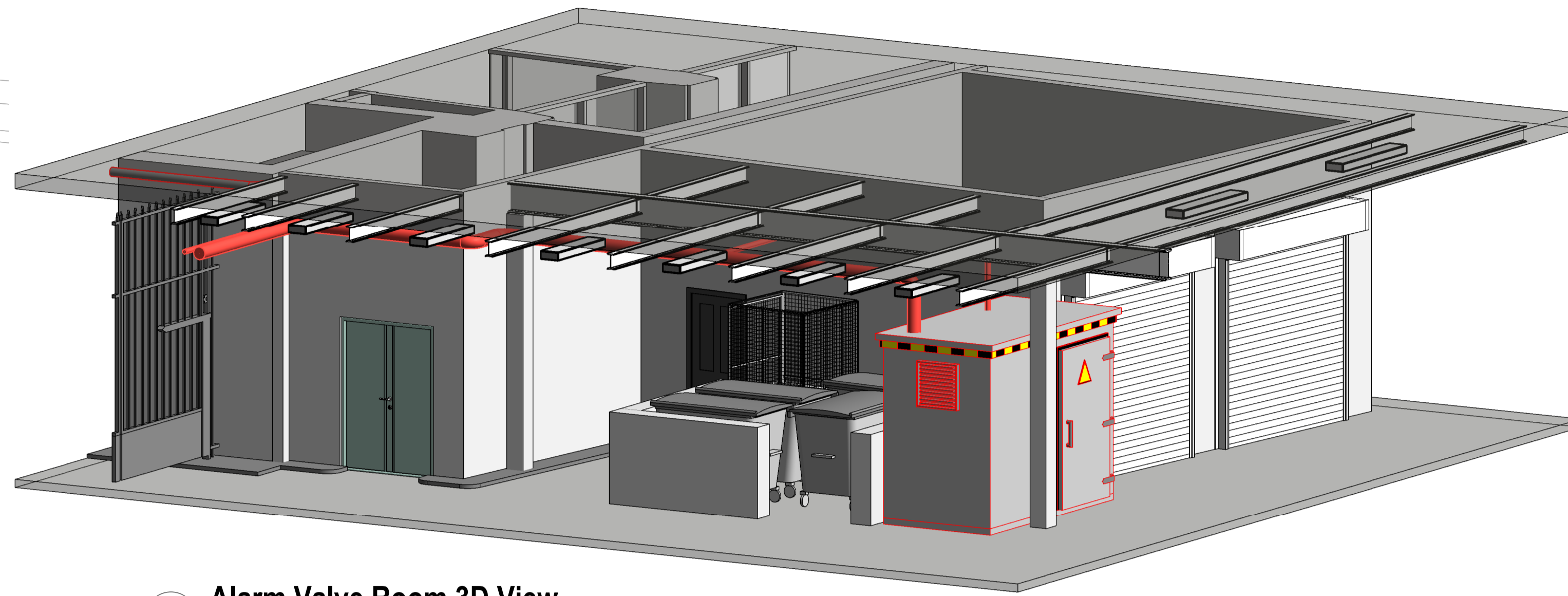
5 Alarm Valve Room 3D View
