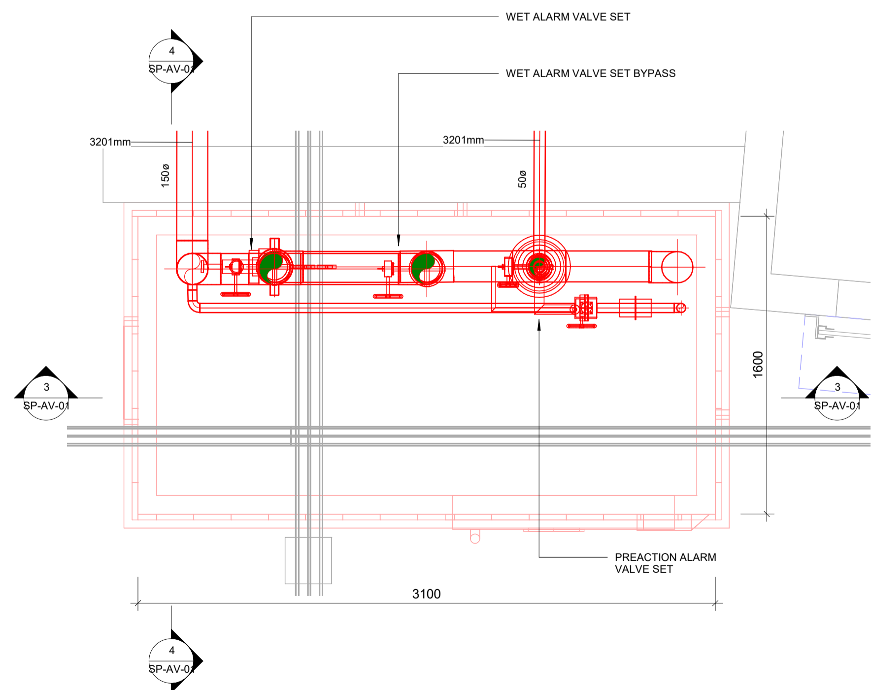
2 Service Yard Alarm Valve Room Floor Plan 1:20
