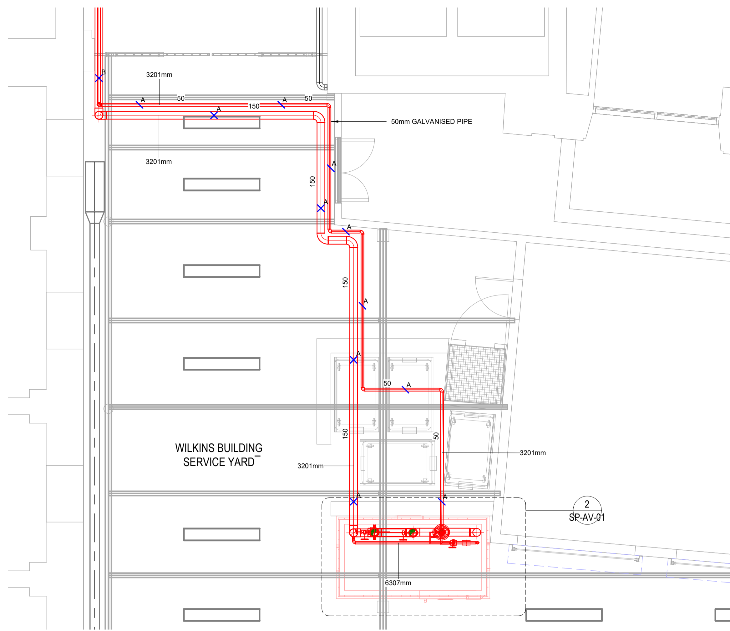
1 Service Yard Alarm Valve Room Layout 1:50
