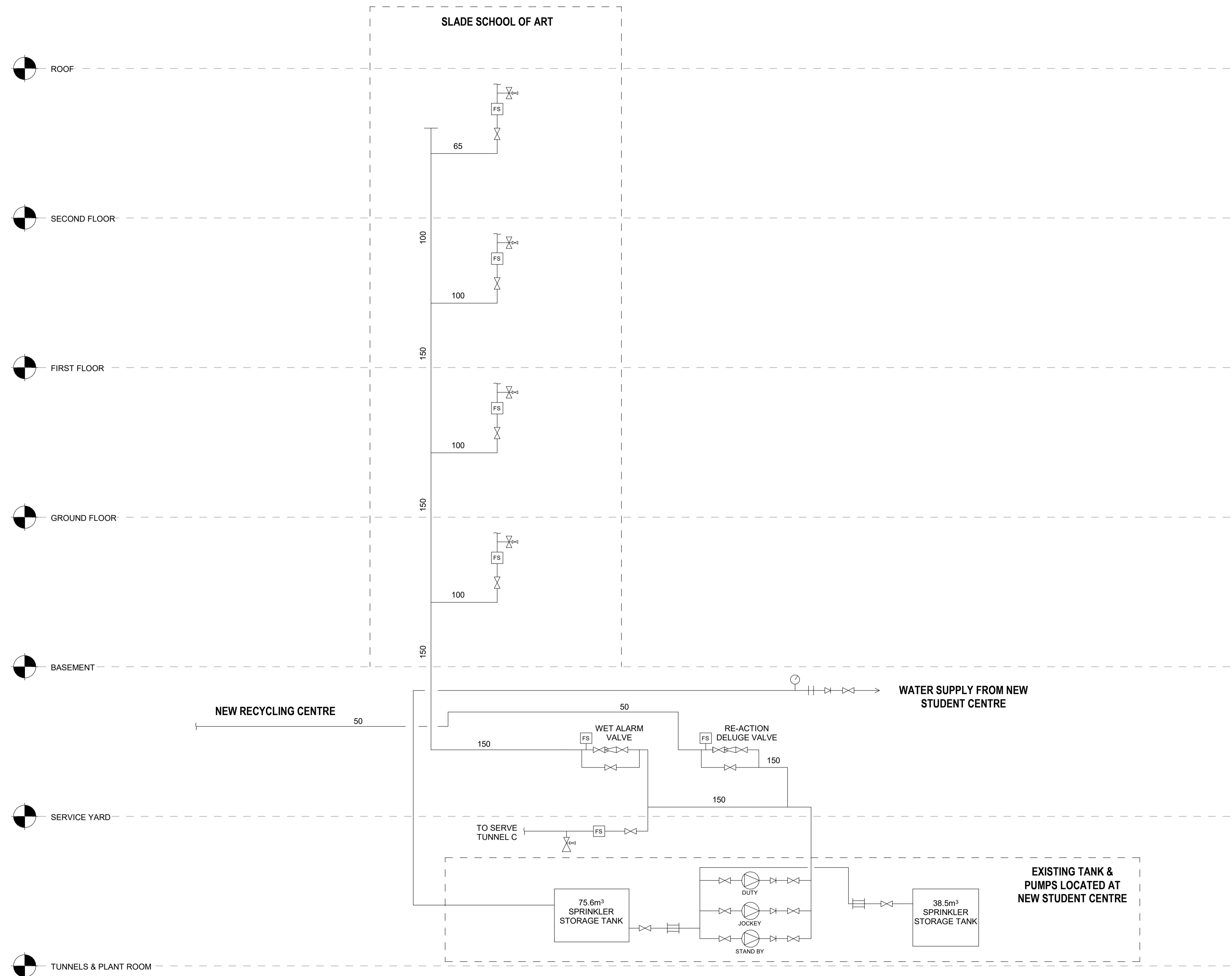
1 Slade School of Art Sprinkler Schematic 1 : 1
