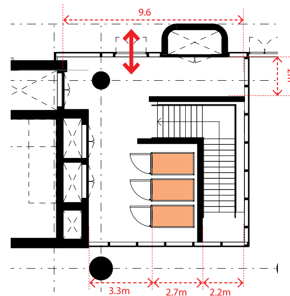
Cycle Store Entrance - Ground Floor Plan
