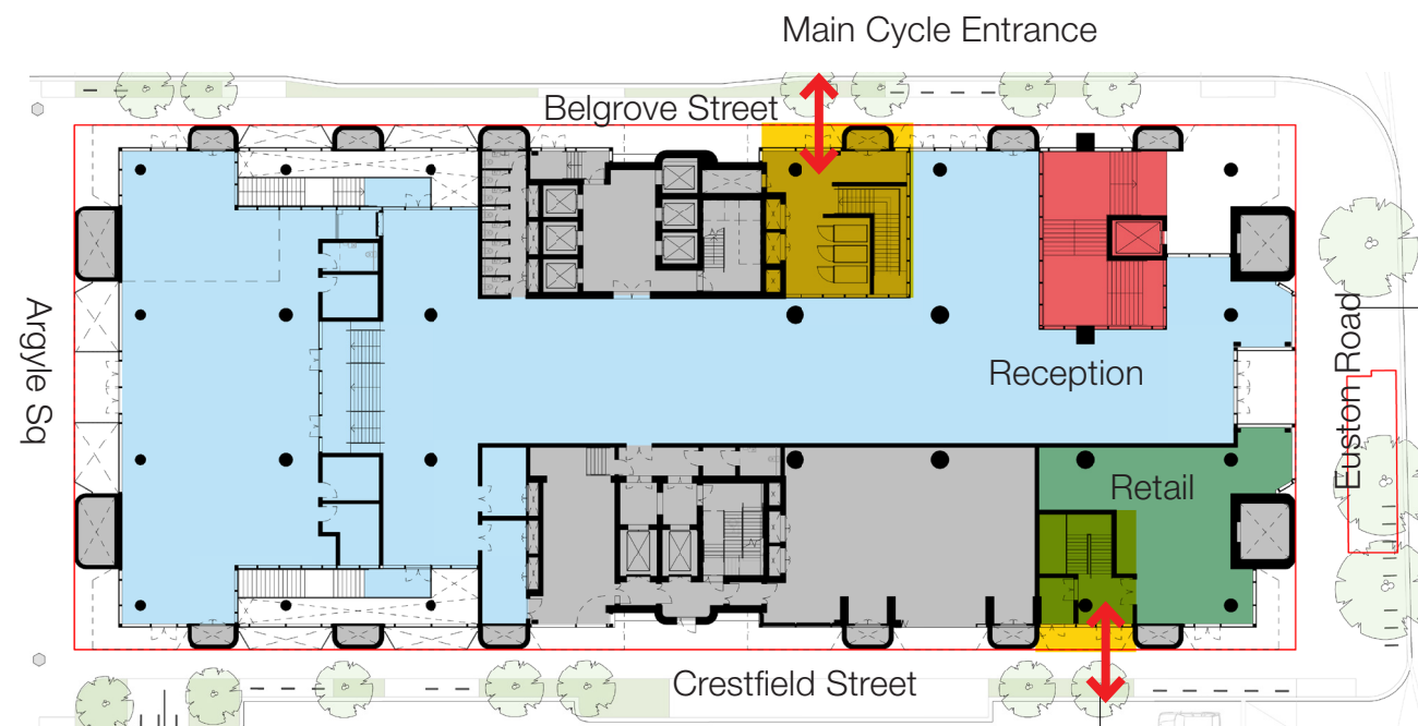
Cycle Store Entrances - Ground Floor Plan
