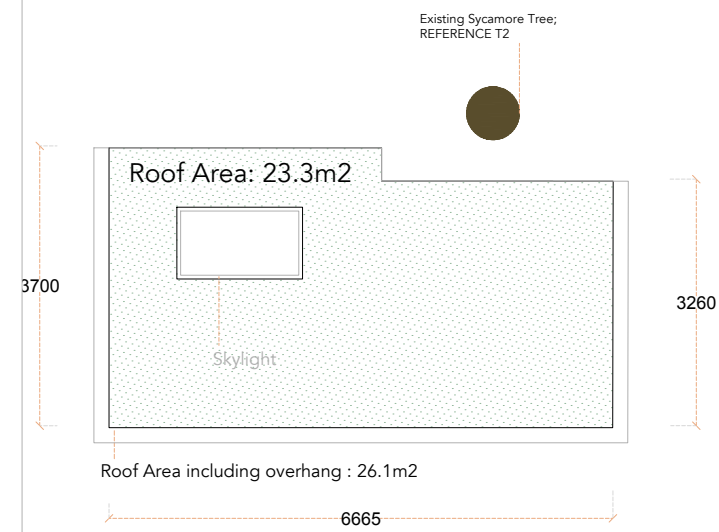
Roof Plan
