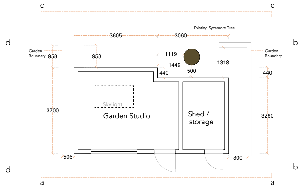
Floor Plan
