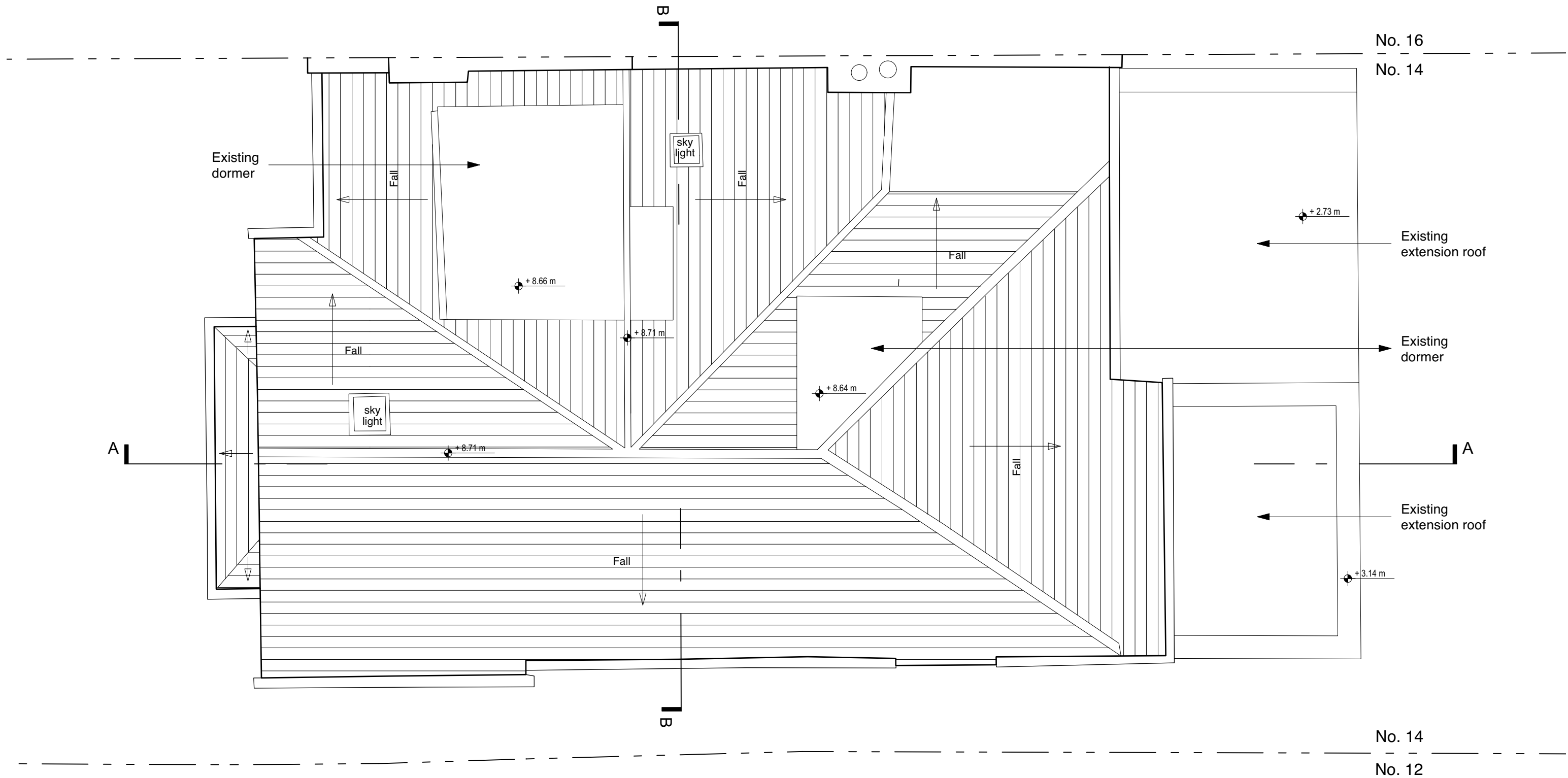
1 EXISTING ROOF PLAN Scale: 1:50
