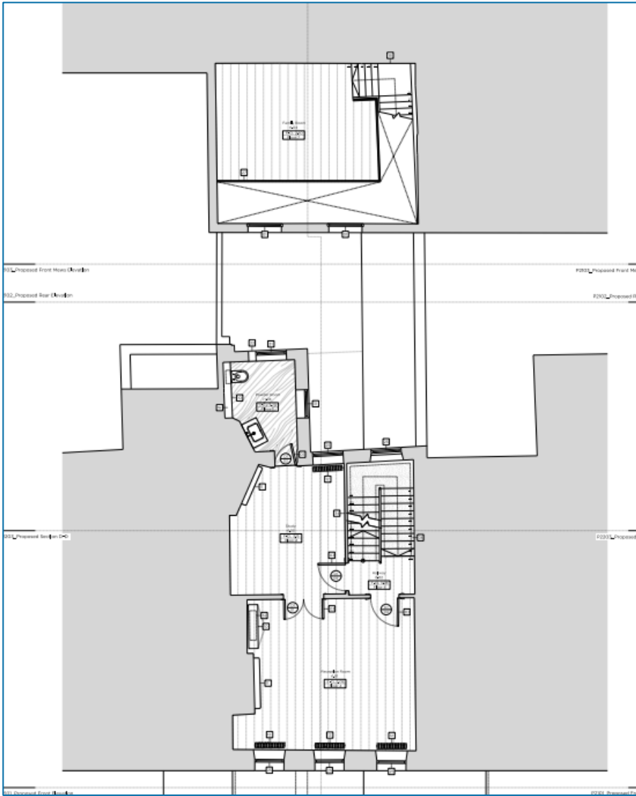
Figure 4: Proposed first floor
