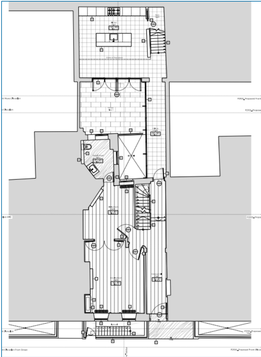
Figure 3: Proposed ground floor
