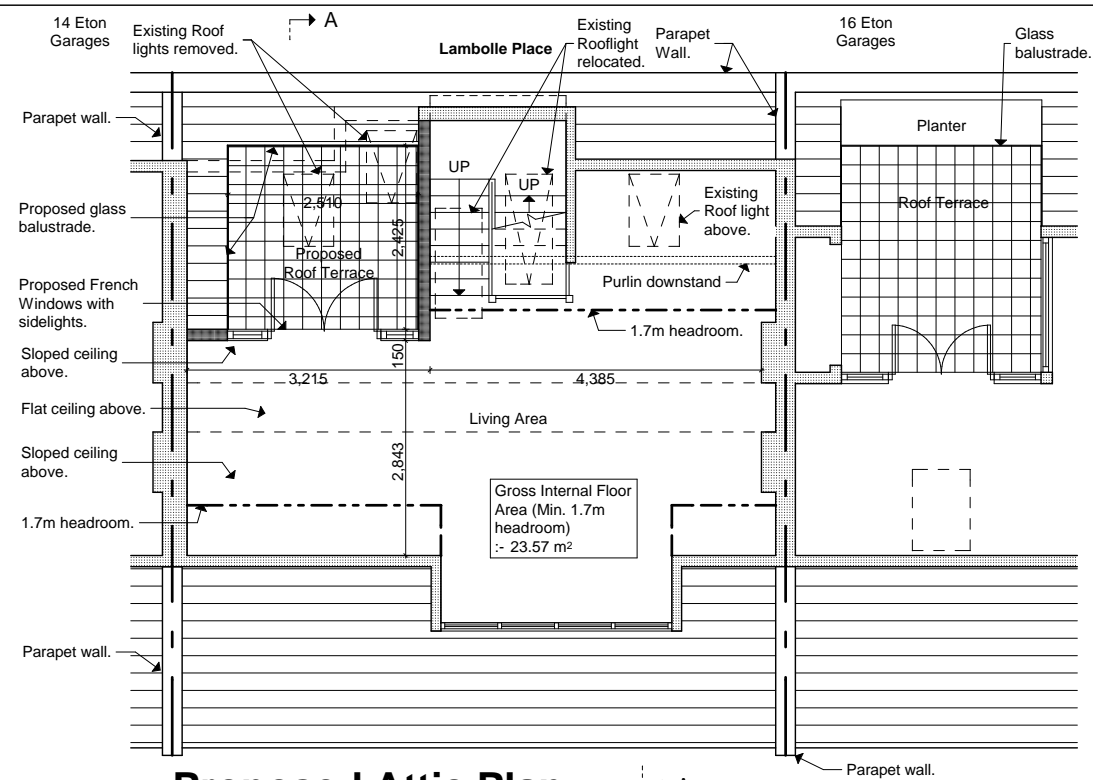
Proposed Attic Plan
