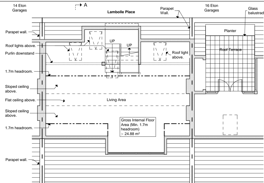
Existing Attic Plan
