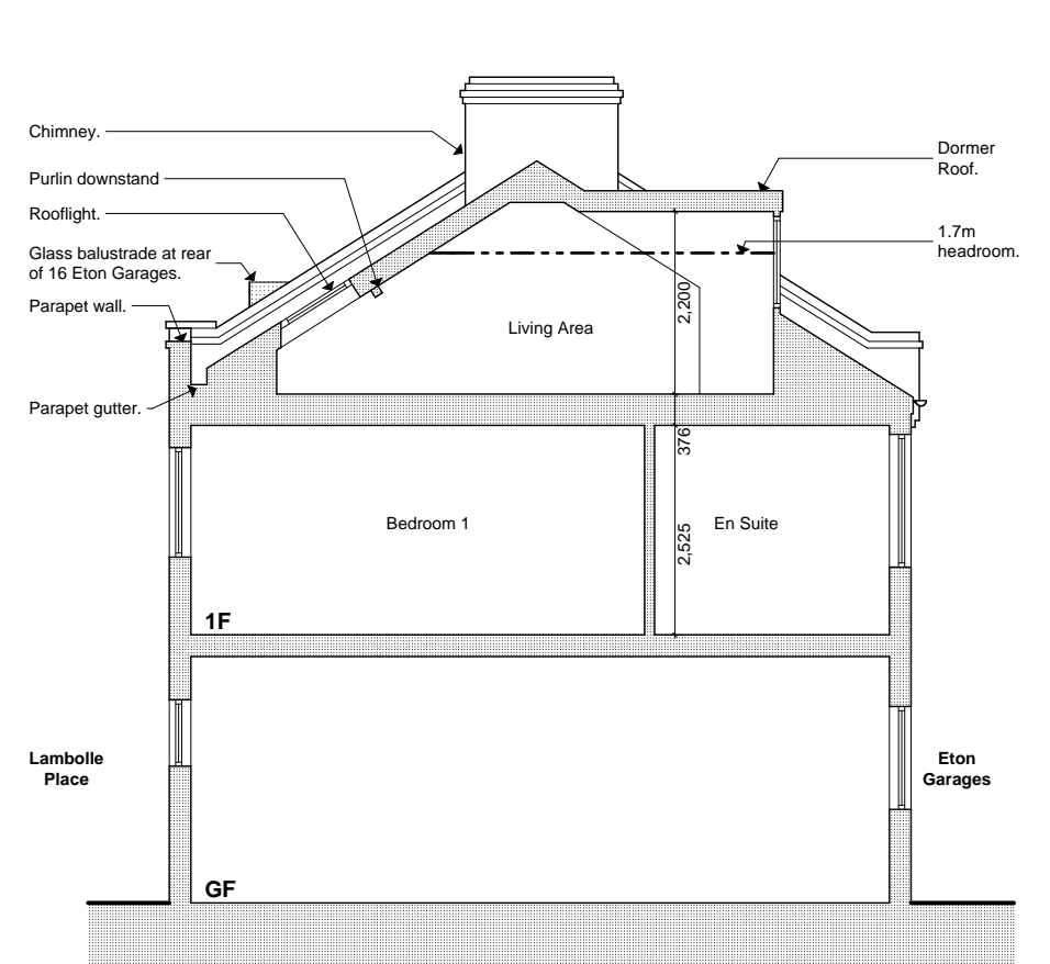
Existing Section A-A
