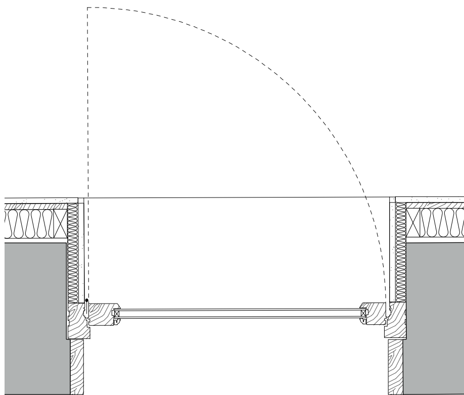
DOOR TYPE 01: HARDWOOD FRAME DOOR - DOUBLE GLAZED - ALL GLAZING TO TO BE SPECIFIED TO ACHIEVE A THERMAL RESISTANCE OF MIN. 1.60W/m2K.
