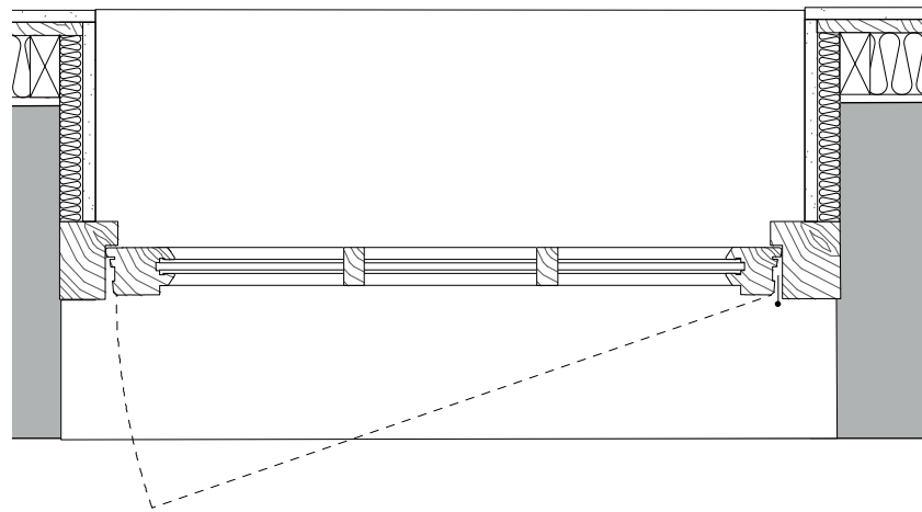
WINDOW TYPE 06: REPLACEMENT SINGLE CASEMENT TOP AND SIDE HUNG OPENABLE - HERITAGE STYLE DOUBLE GLAZED - ALL GLAZING TO TO BE SPECIFIED TO ACHIEVE A THERMAL RESISTANCE OF MIN. 1.60W/m2K.
