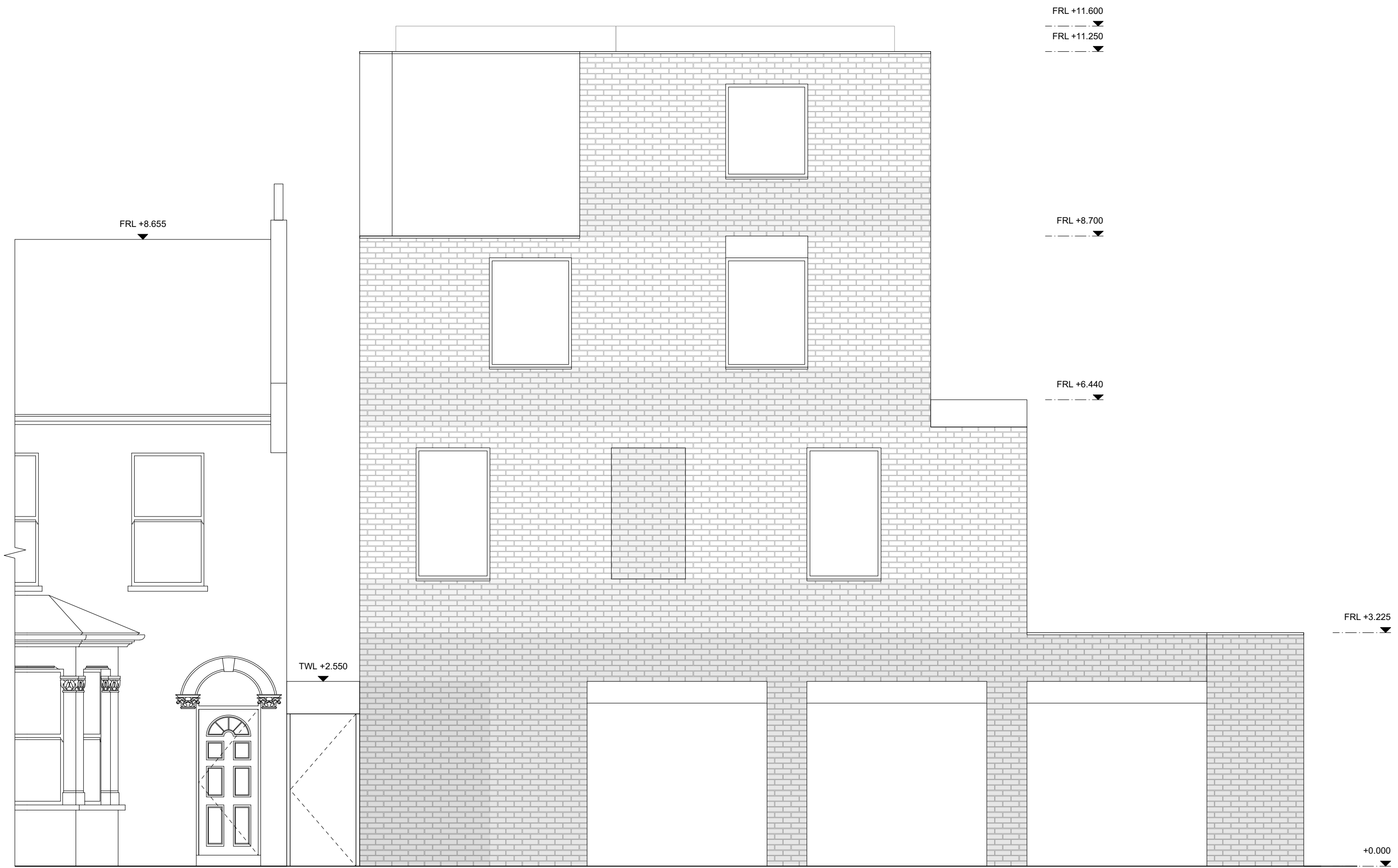
1 PROPOSED FRONT ELEVATION 1:50@A3
