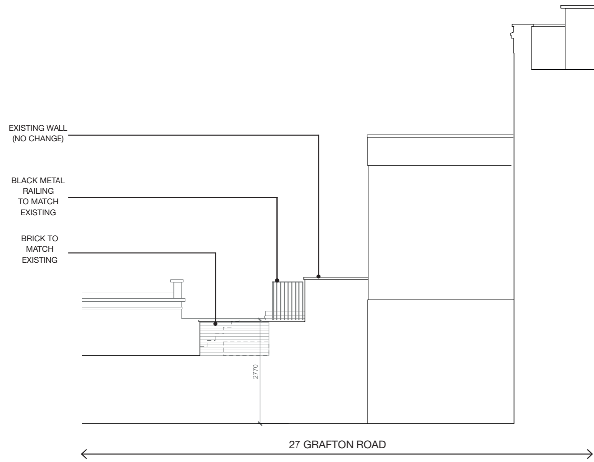
2 | PROPOSED SOUTH ELEVATION
