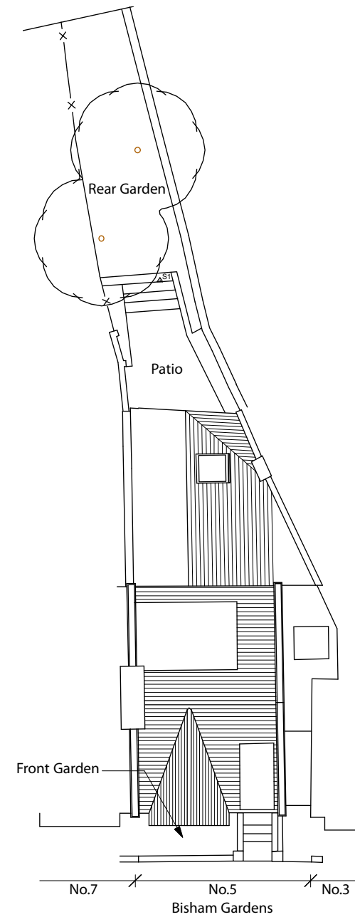
Proposed Site Block Plan
