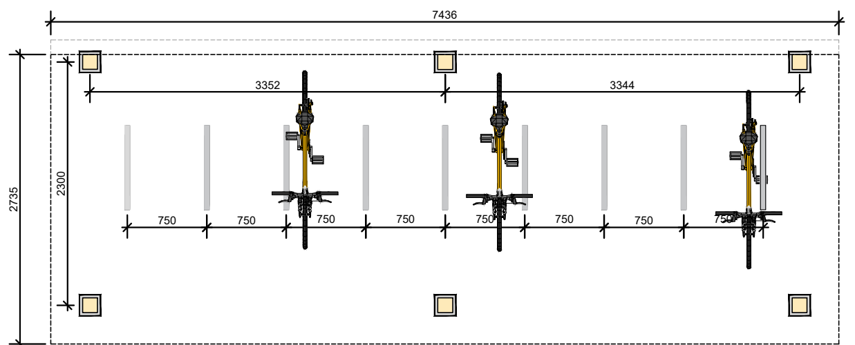
Floor Plan
