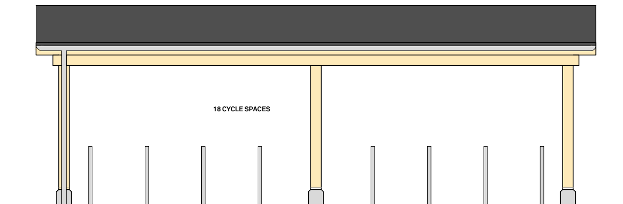
Rear Elevation
