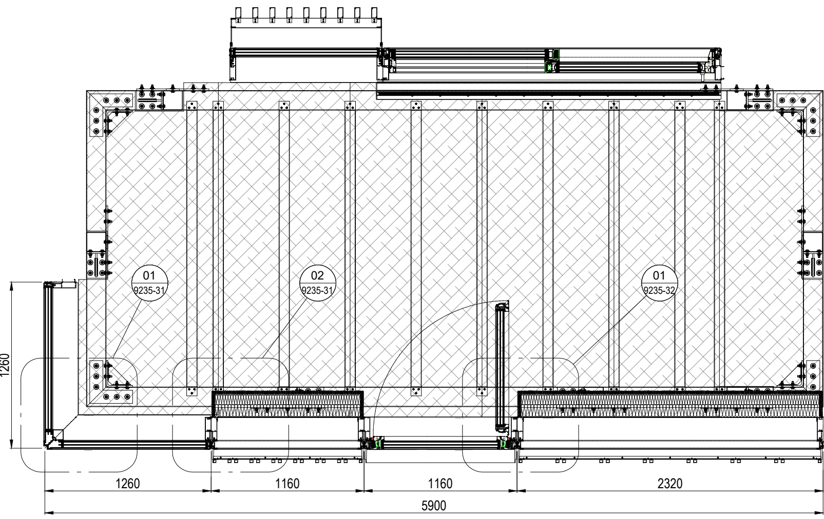
SECTION G-G
