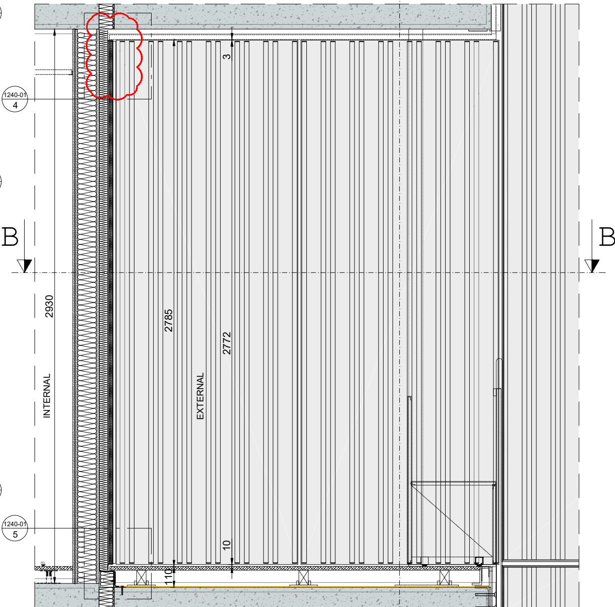
PARTIAL ELEVATION
