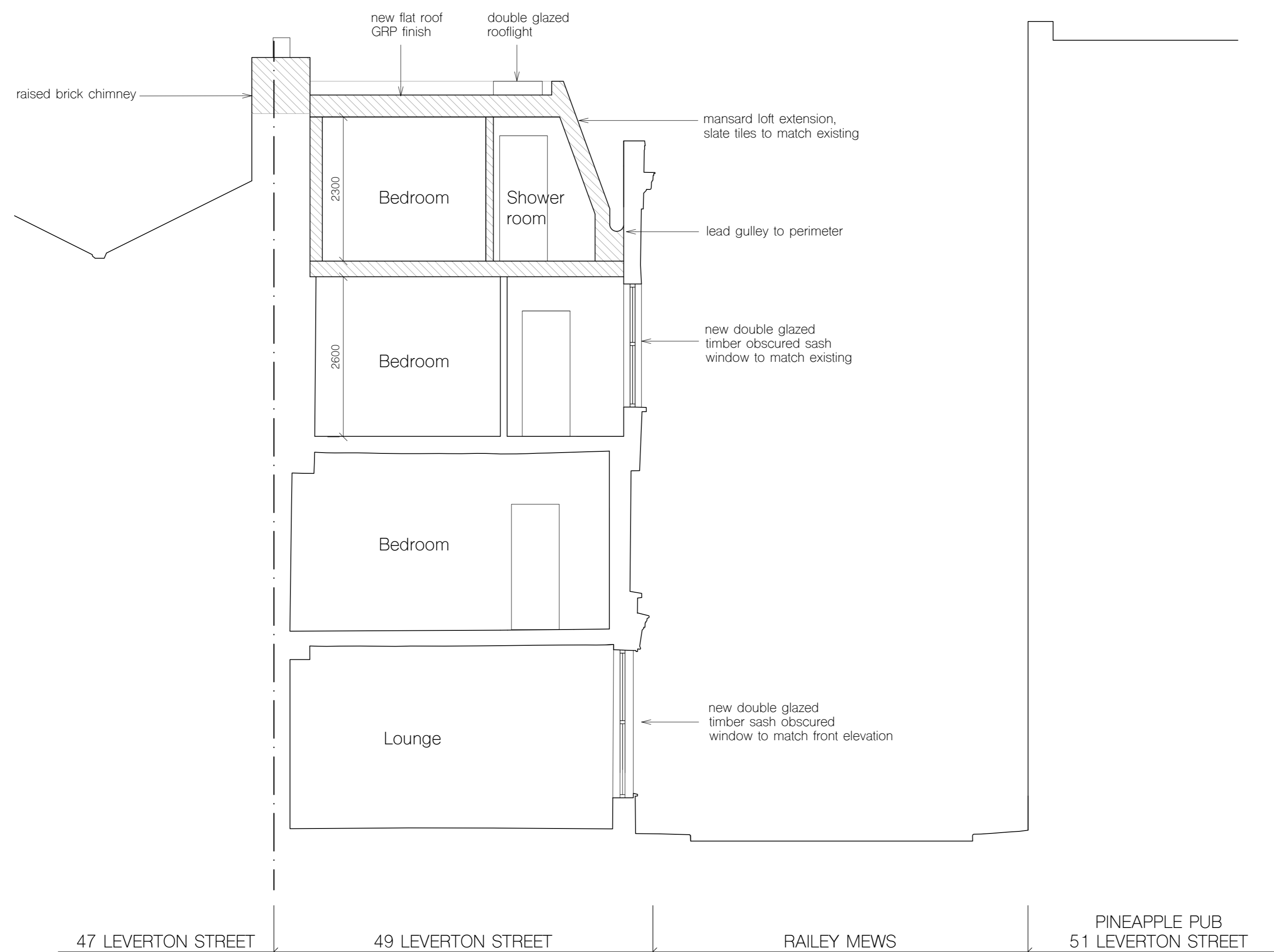
1 Proposed section CC
