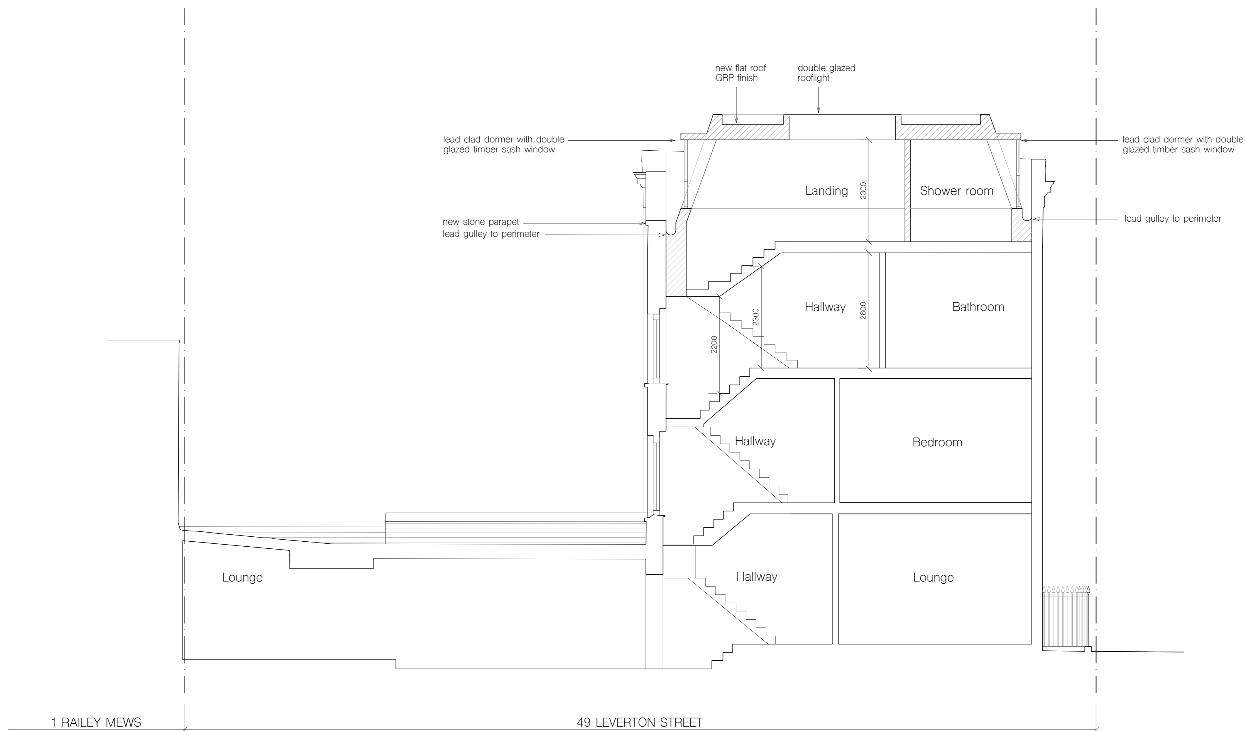
1 Proposed section BB
