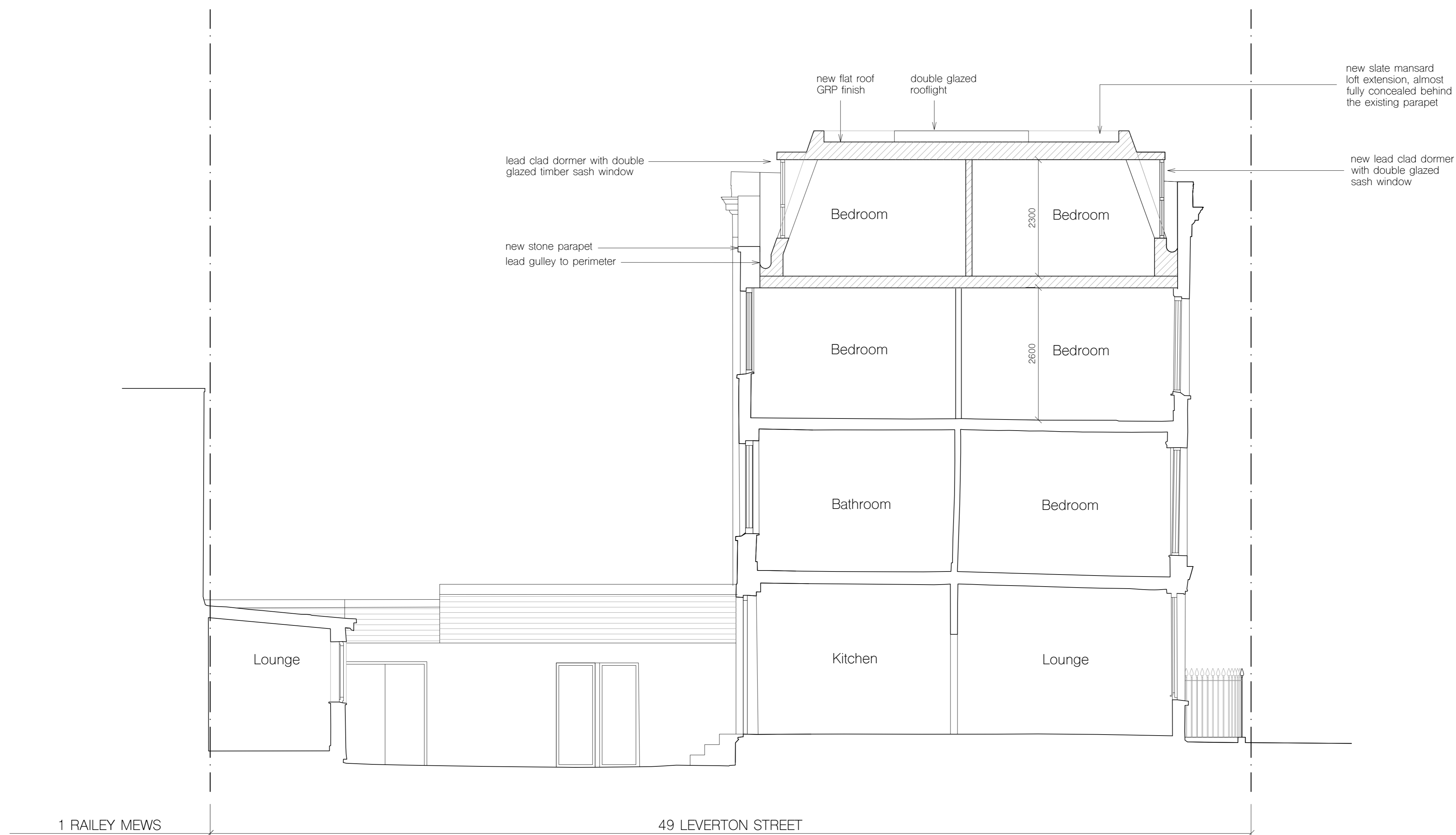
1 Proposed section AA
