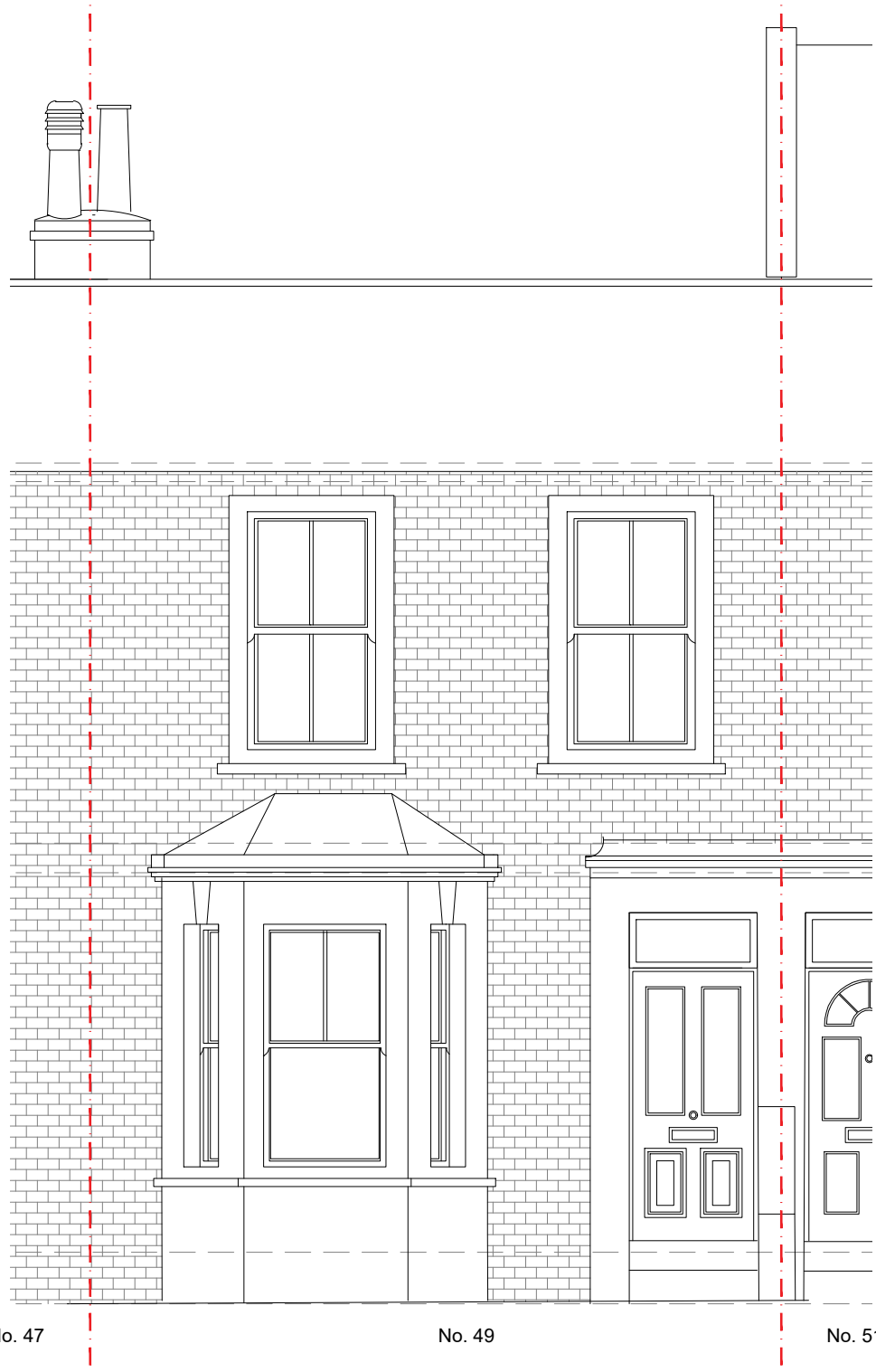
01 Existing Front Elevation 10.271 Scale 1:50 @ A3
