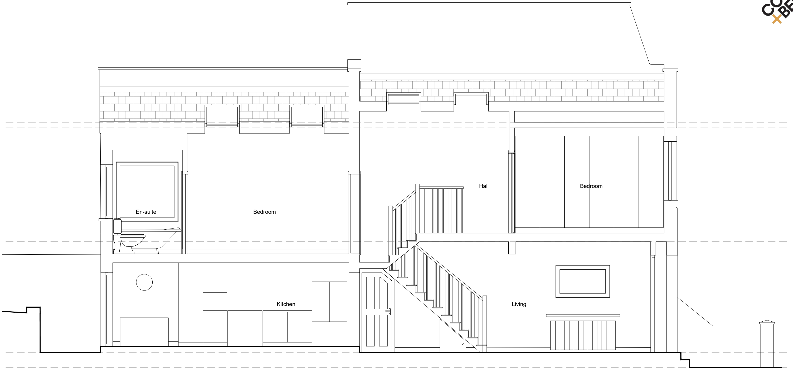
01 Existing Section AA 10.251 Scale 1:50 @ A3
