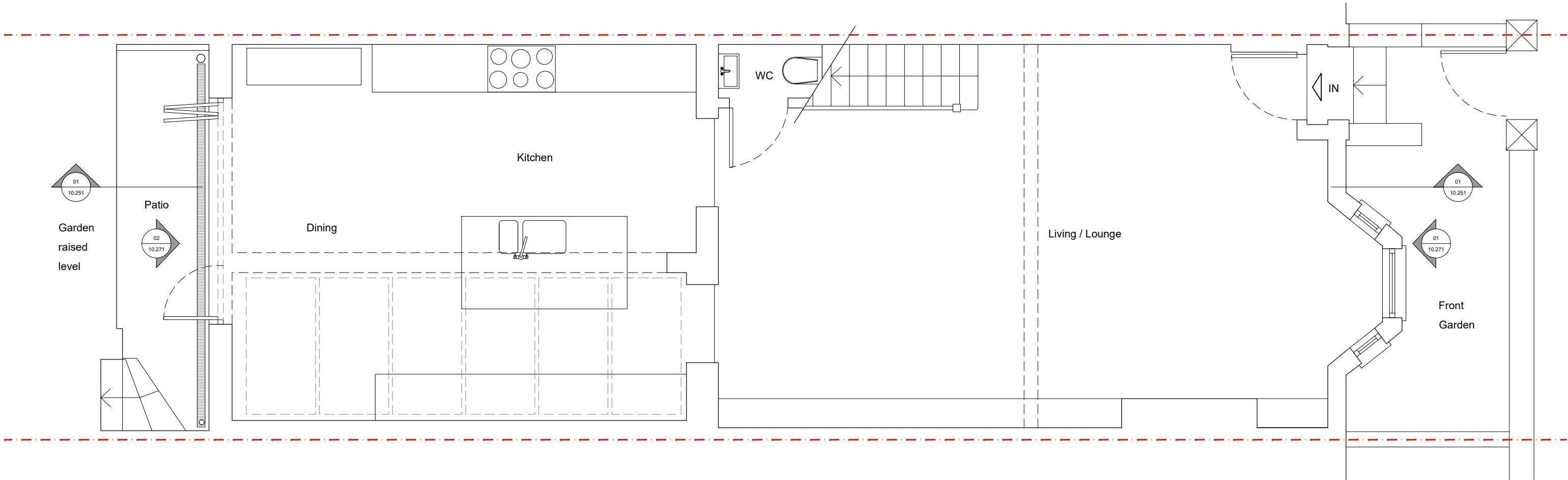
01 Existing Ground Floor Plan 10.201 Scale 1:50 @ A3
