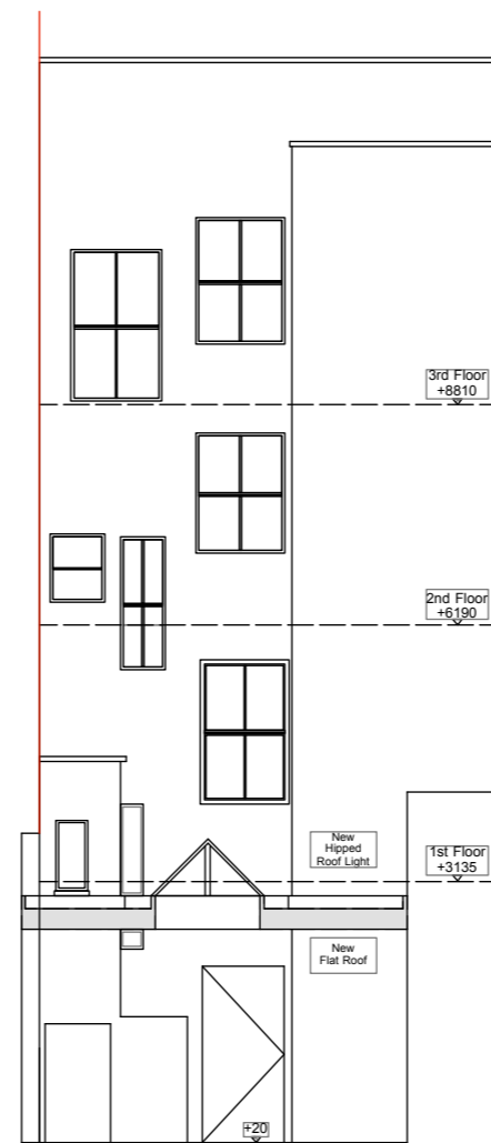
SOUTH ELEVATION TO REAR
