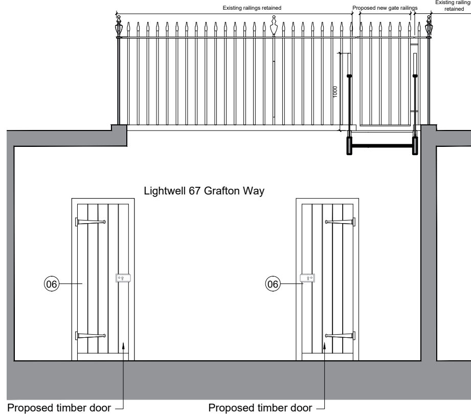
2 Section E-E (as viewed from lightwell) 1:100
