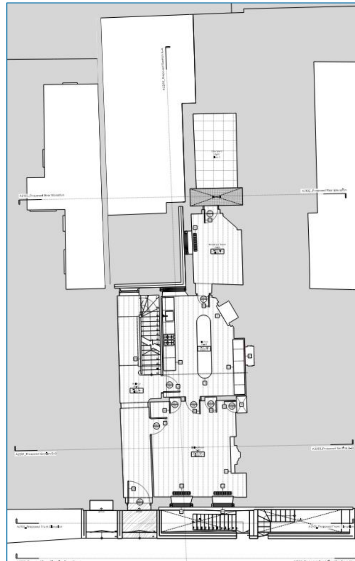
Figure 3: Proposed ground floor
