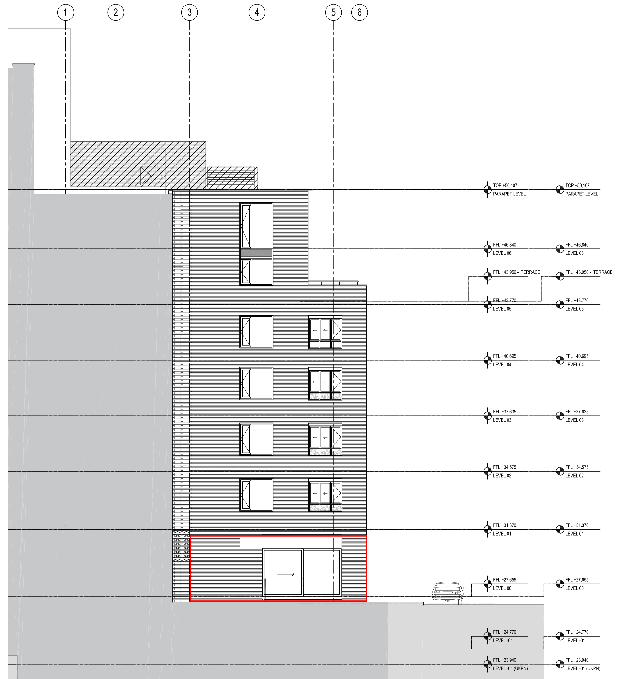
1 Poets Park Elevation (Chitty Street) 1 : 100
