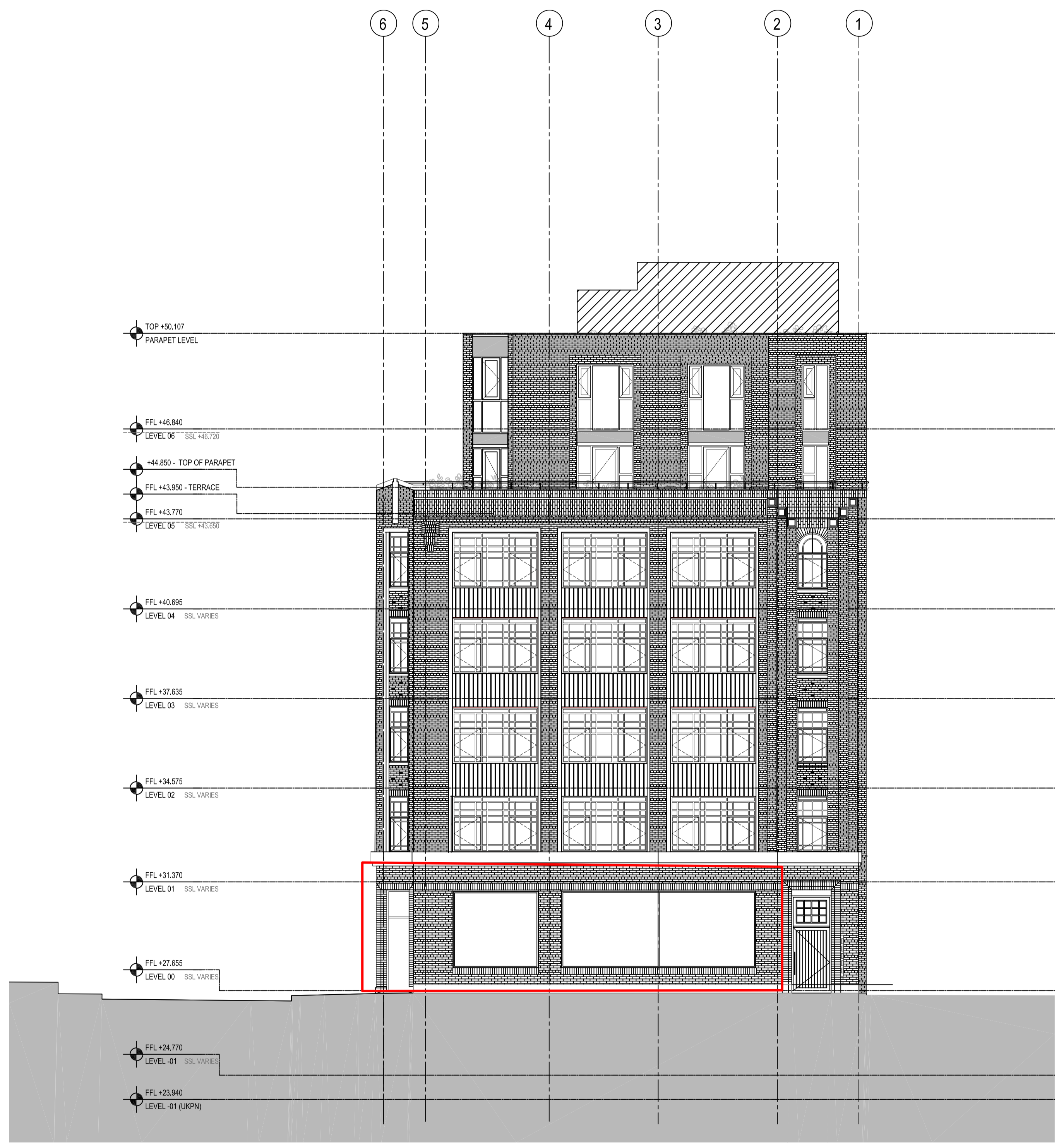
1 Whitfield Street Elevation 1 : 100
