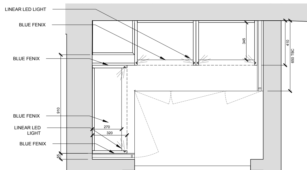
01 Room 8 - Kitchenette - Plan D scale 1:20 @A3
