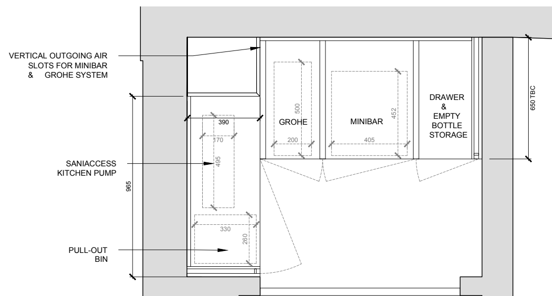
01 Room 8 - Kitchenette - Plan D scale 1:20 @A3
