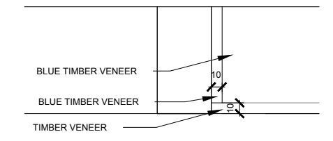
04 TV Joinery - Detail C scale 1:5 @A3
