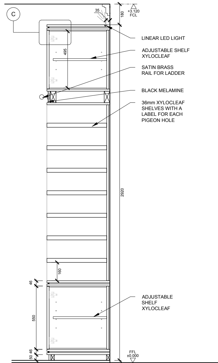
01 Room 3 - Joinery around Doors - Section B scale 1:20 @A3
