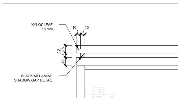
02 Room 3 - Joinery around Doors - Detail C scale 1:5 @A3
