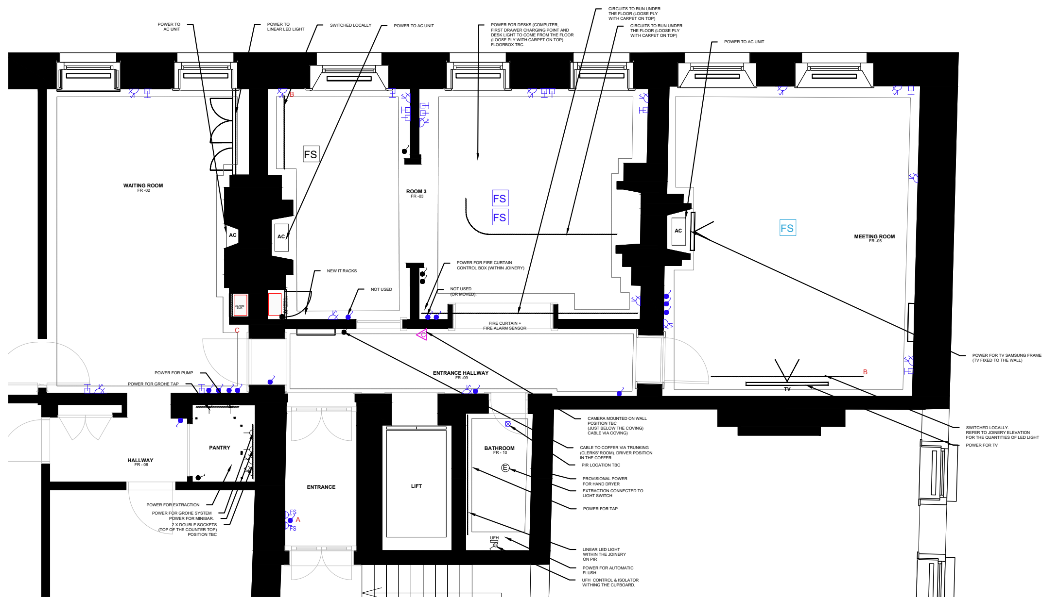
01 Proposed Small Power Layout scale 1:75 @A3
