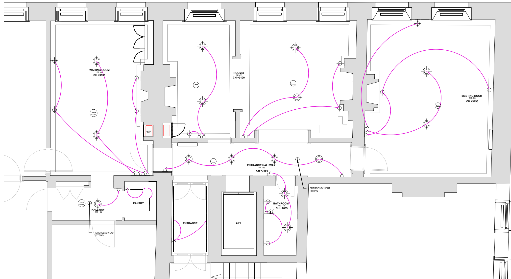
01 Existing RCP & Lighting Layout scale 1:75 @A3
