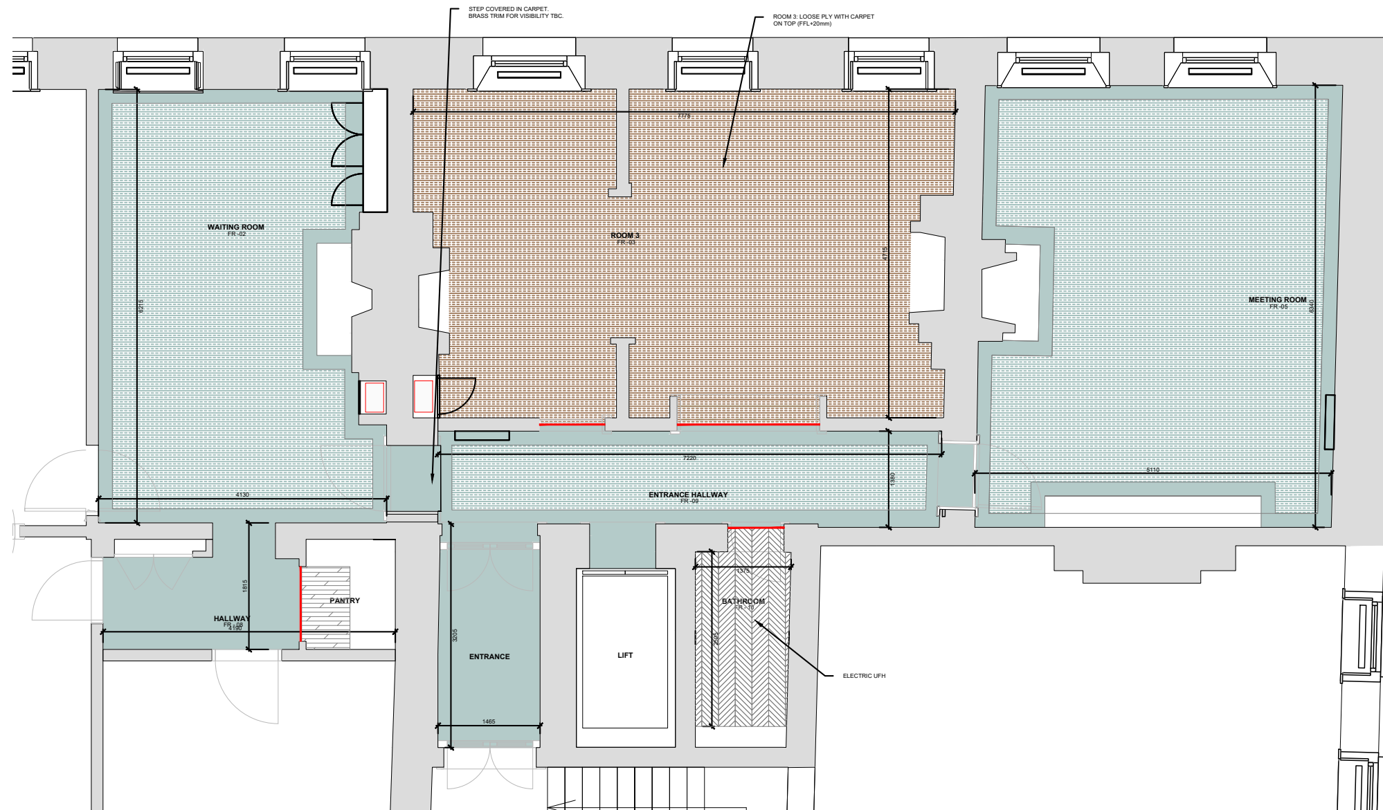
01 Floor Finishes Layout scale 1:75 @A3
