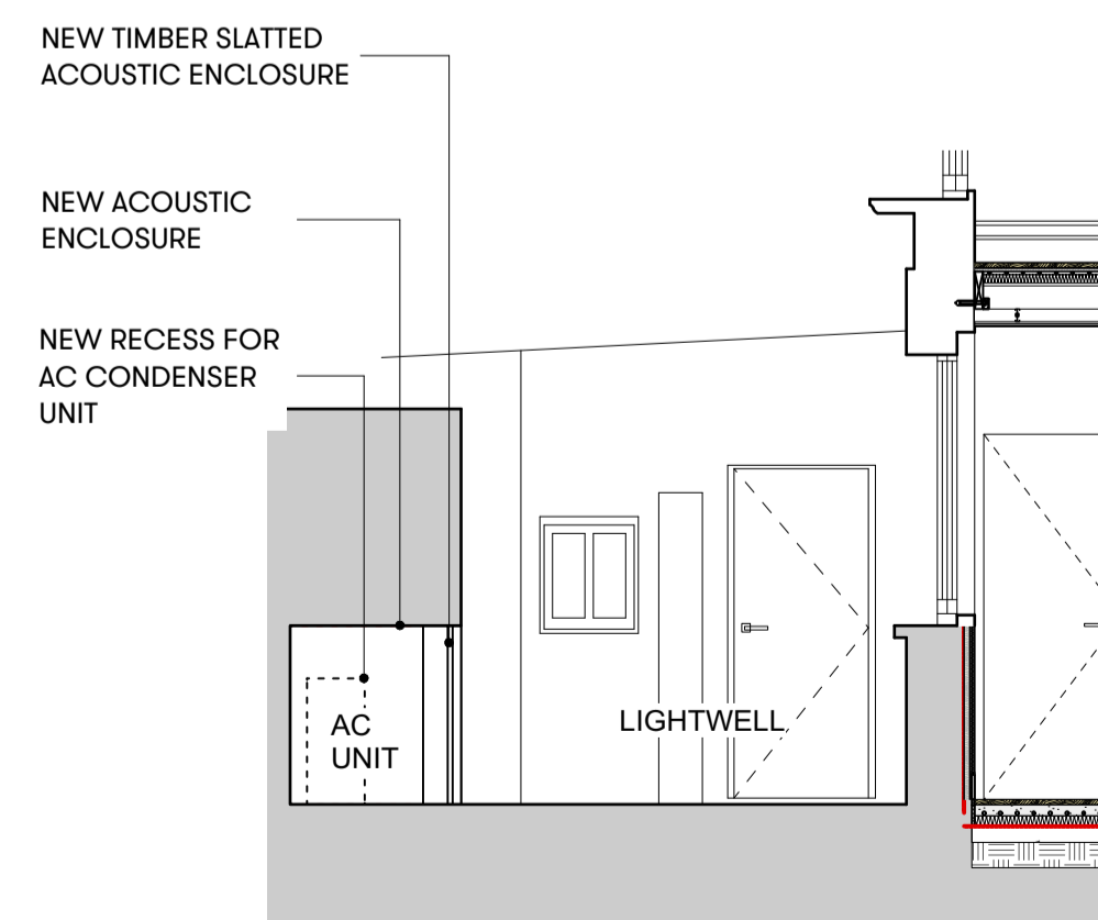
08 Proposed Section 1:50 @ A1
