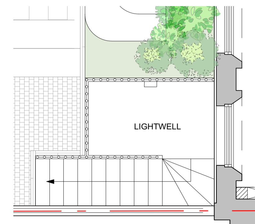
07 Proposed Upper GF Plan 1:50 @ A1
