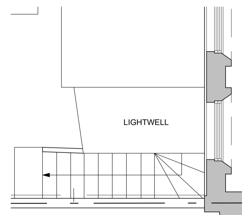
03 Existing Upper GF Plan 1:50 @ A1
