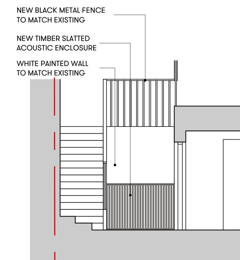
09 Proposed Elevation 1:50 @ A1
