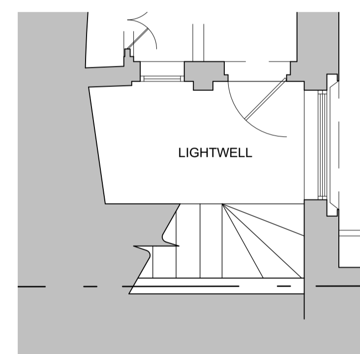
02 Existing Lower GF Plan 1:50 @ A1
