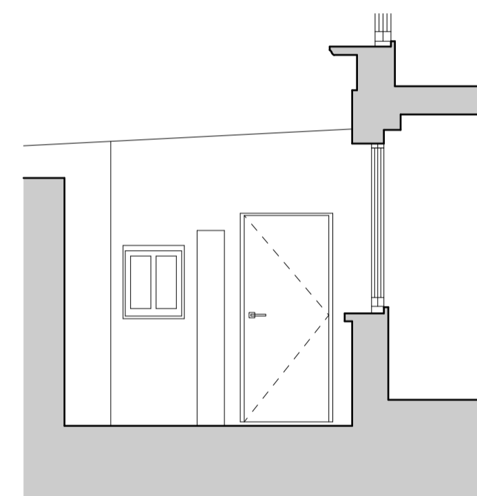
04 Existing Section 1:50 @ A1
