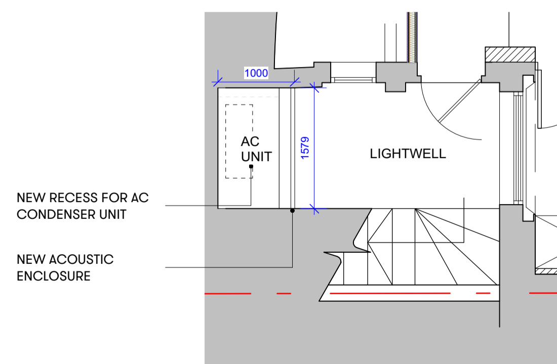
06 Proposed Lower GF Plan 1:50 @ A1
